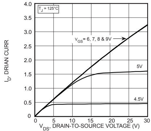
Figure 2, Output Characteristics
