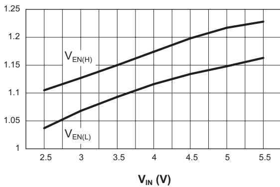
V EN(H) and V EN(L) vs. V IN
