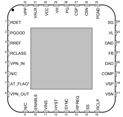
QFN PACKAGE (Top View)
