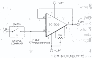
FIGURE 8 - LOW-DRIFT SAMPLE AND HOLD
