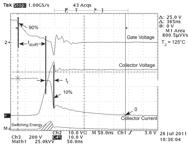
Figure 22, Turn-off Switching Waveforms and Definitions
