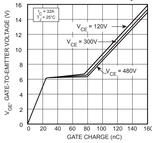
FIGURE 4, Gate charge
