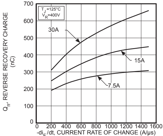
Figure 26. Reverse Recovery Charge vs. Current Rate of Change
