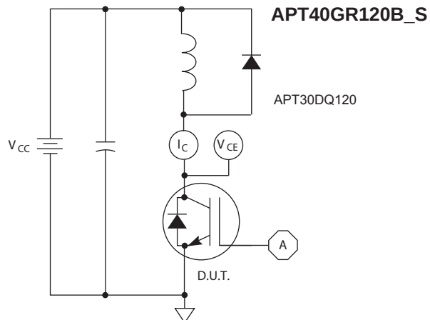
FIGURE 10, Inductive Switching Test Circuit
