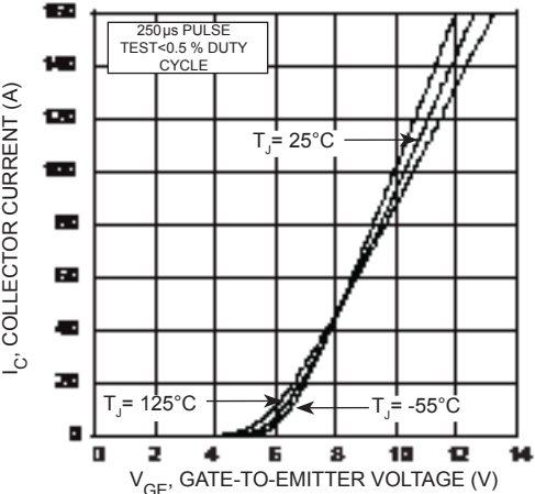
FIGURE 3, Transfer Characteristics
