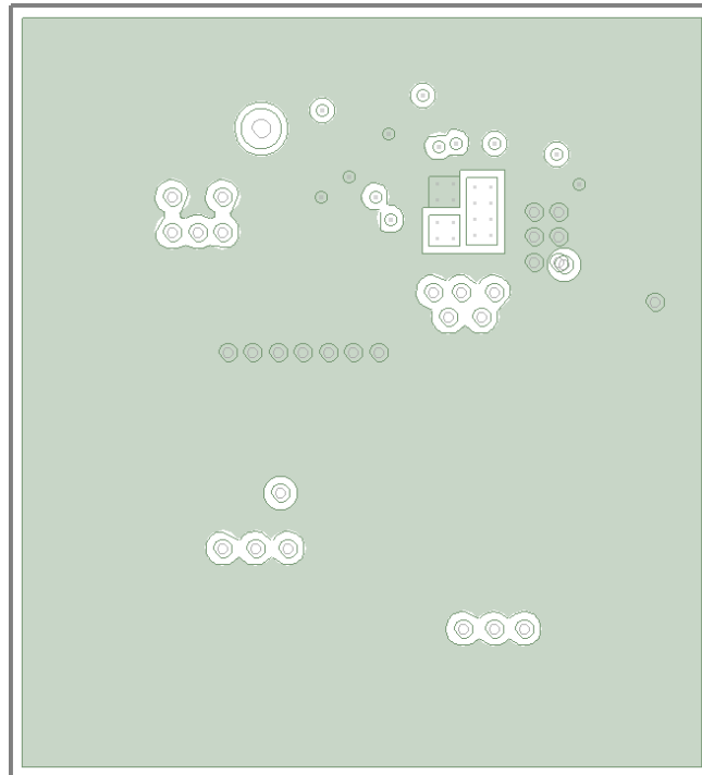
Figure 13. Ground Layer
