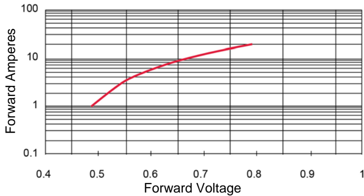
FIGURE 2 1N6841 V_F vs. I_F
