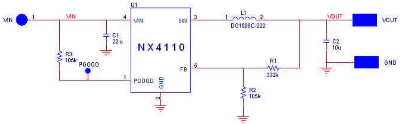
Fig. 19 - Demoboard schematic
