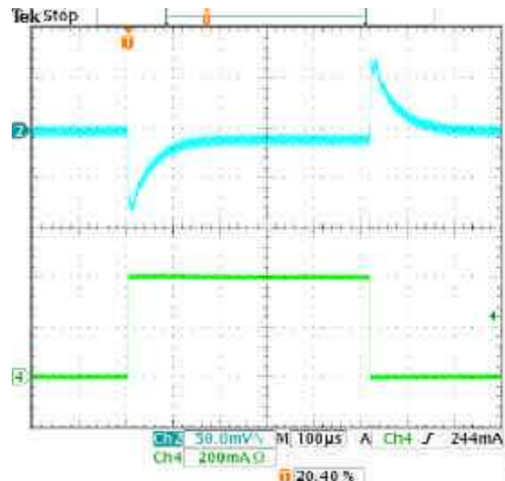
Fig. 11 - Transient response
