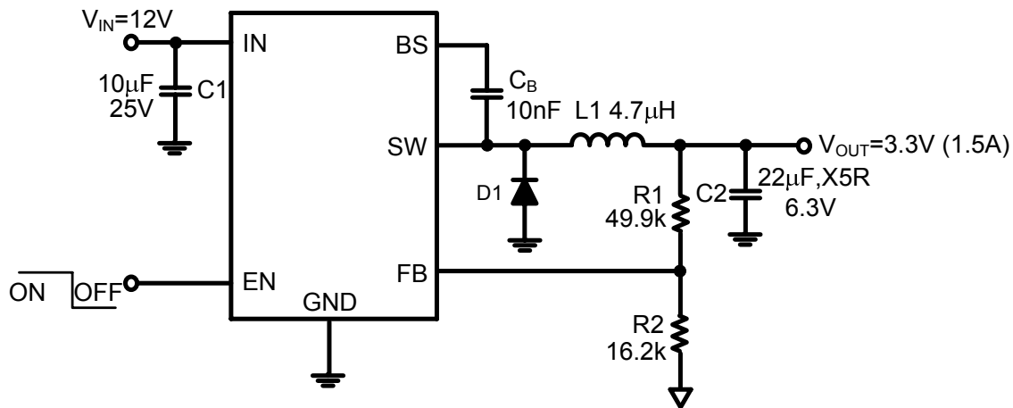
Typical Application
