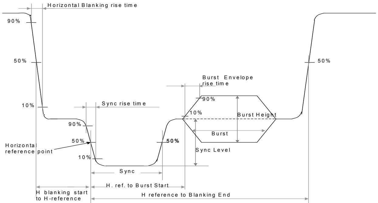
Fig. 15 Synchronizing Signal and Burst Waveform
