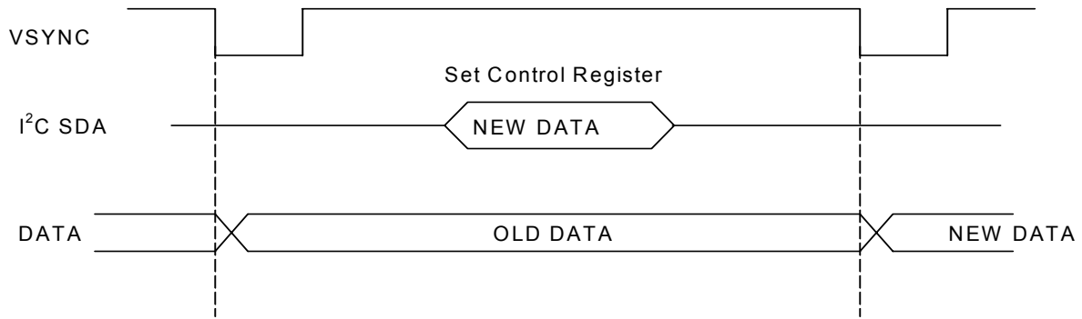
Fig. 8 WSS Data Renewal Timing
