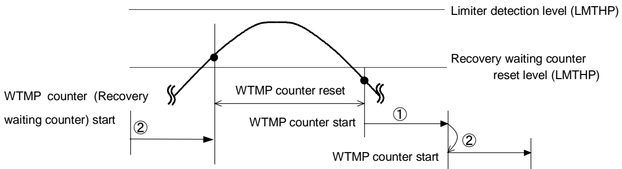
Figure 21: ALC recovery waiting counter
