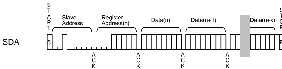
Figure 16: WRITE Operation
