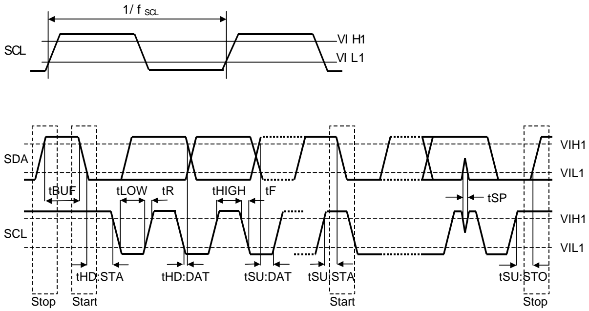
Figure 3: I2C Interface Timing
