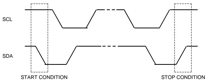
Figure 11: START and STOP conditions
