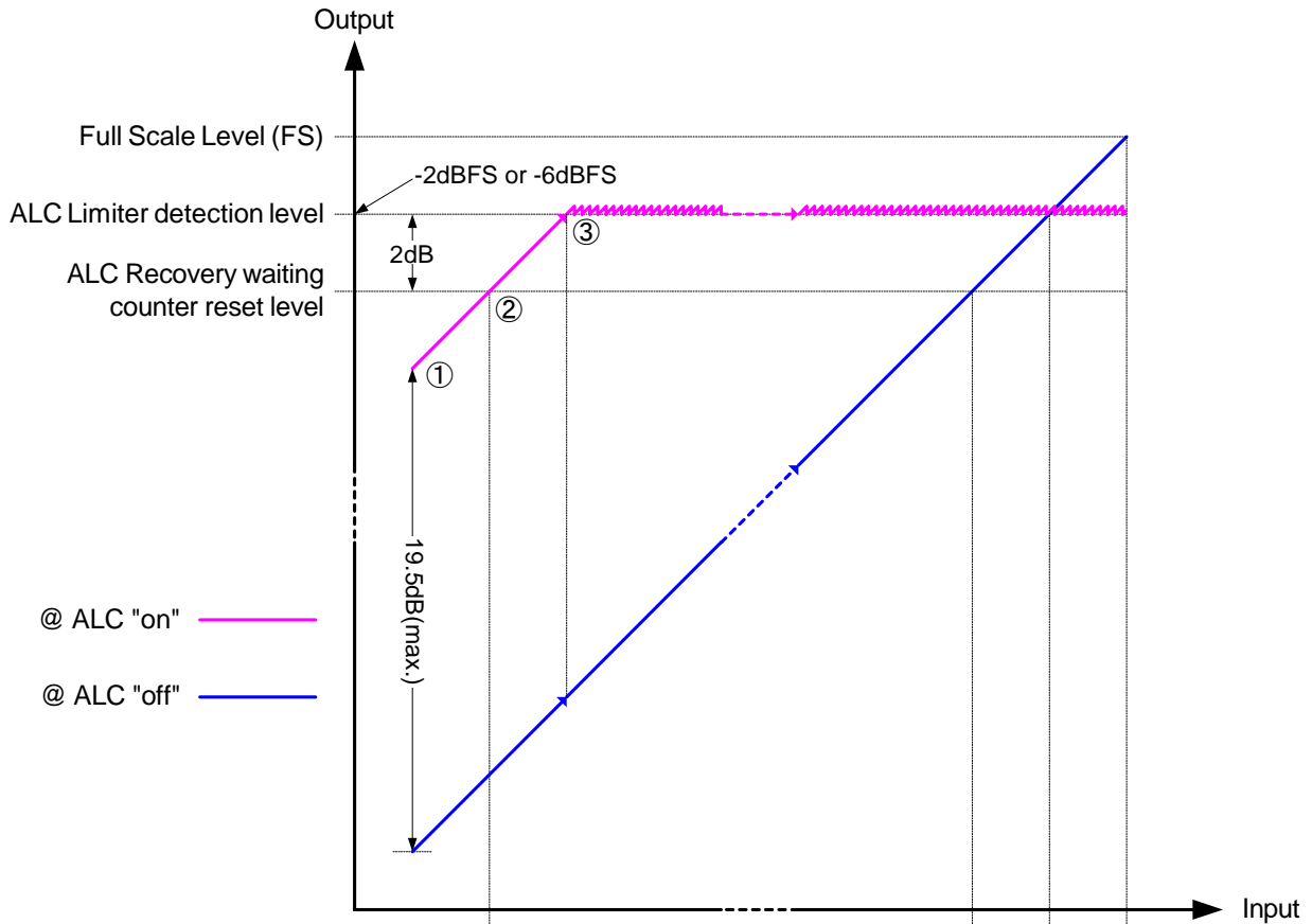
Figure 23: Input/Output characteristic (1)
