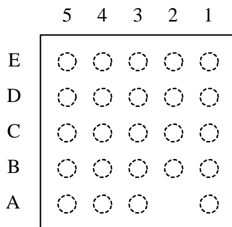
Figure 2: Pin Location (Top View)
