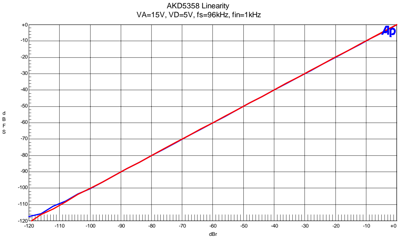
Figure 11. Linearity
