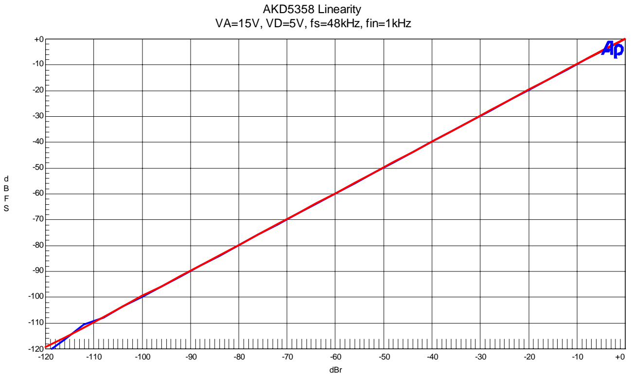
Figure 3. Linearity
