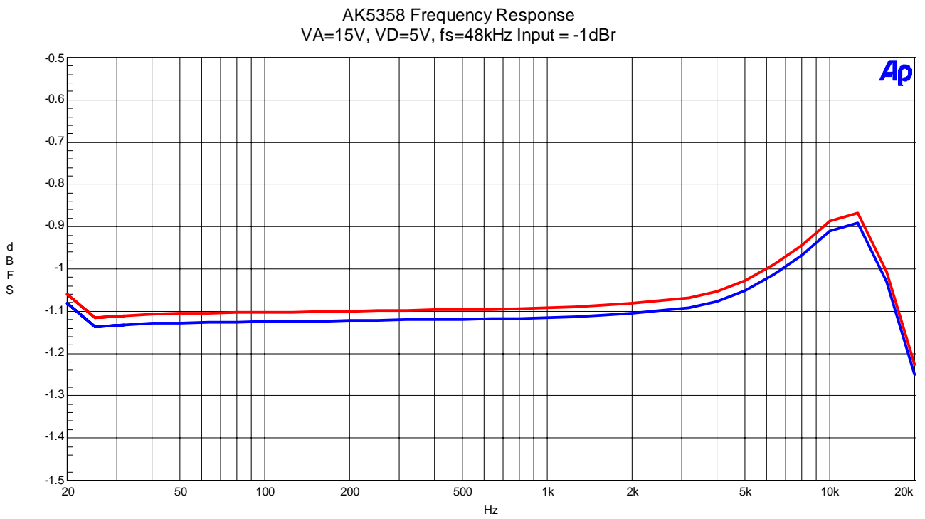
Figure 4. Frequency Response
