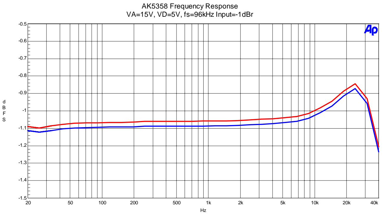
Figure 12. Frequency Response
