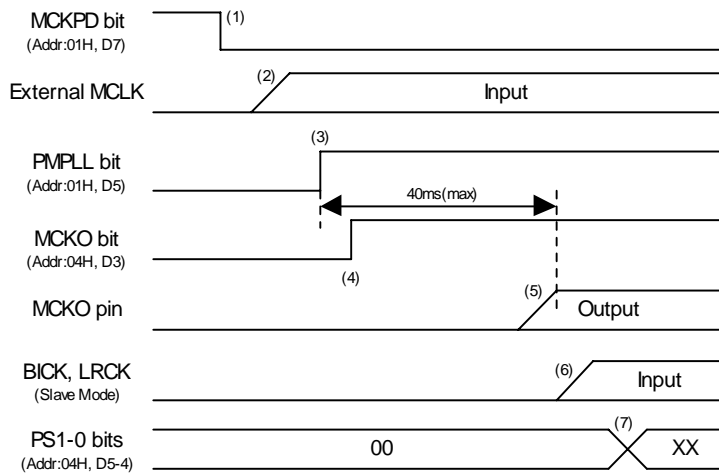
Figure 47. Clock Set Up Sequence(3)
