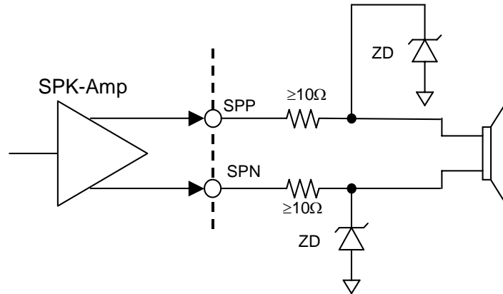
Figure 34. Circuit of Speaker Output(Load Capacitance > 30pF)
