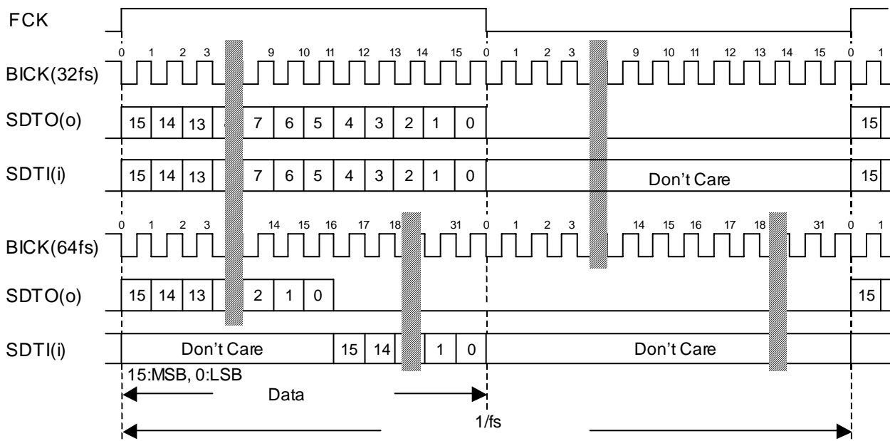
Figure 26. Mode 1 Timing
