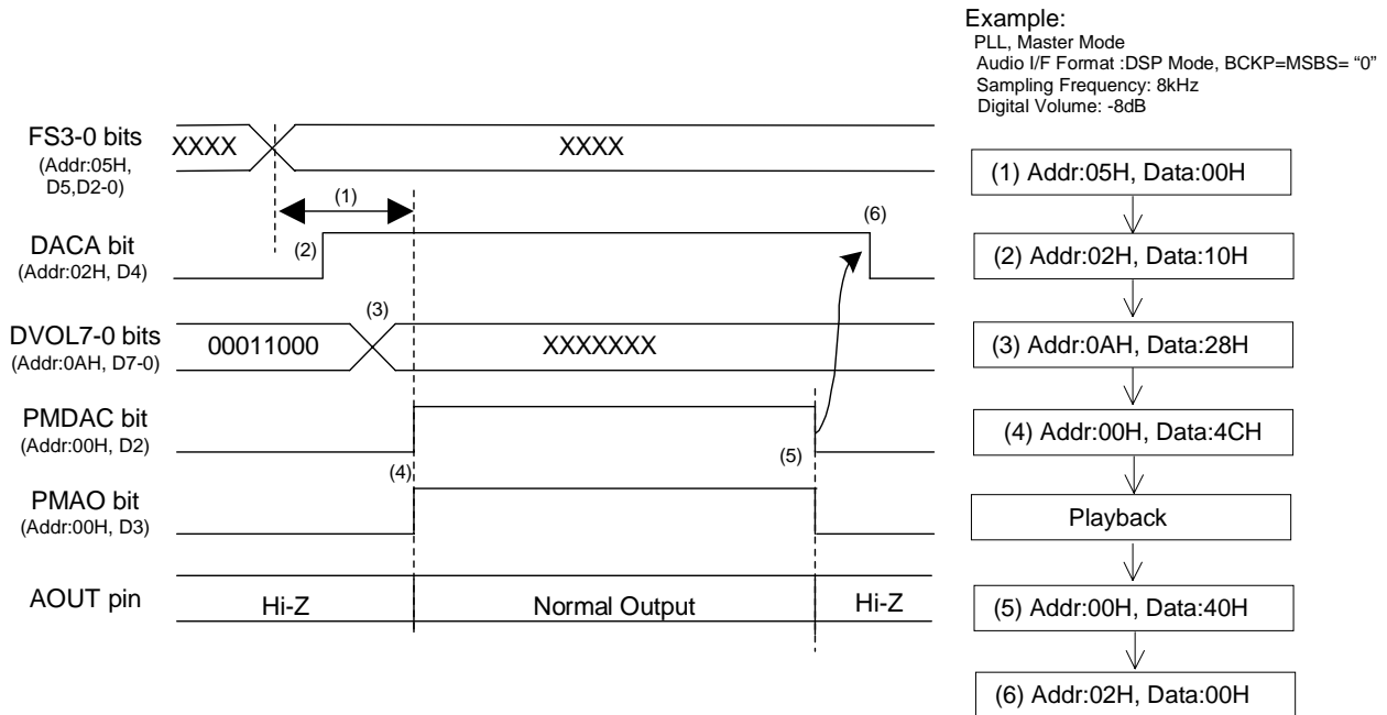
Figure 50. Mono Lineout Sequence
