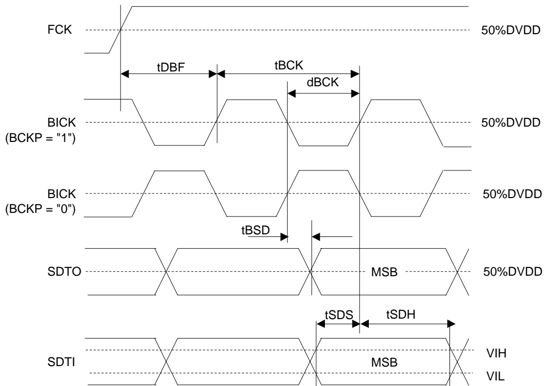
Figure 4. Audio Interface Timing (PLL Master mode & DSP mode: MSBS bit="1")
