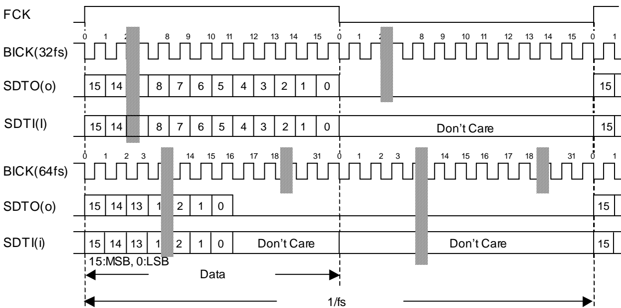
Figure 27. Mode 2 Timing
