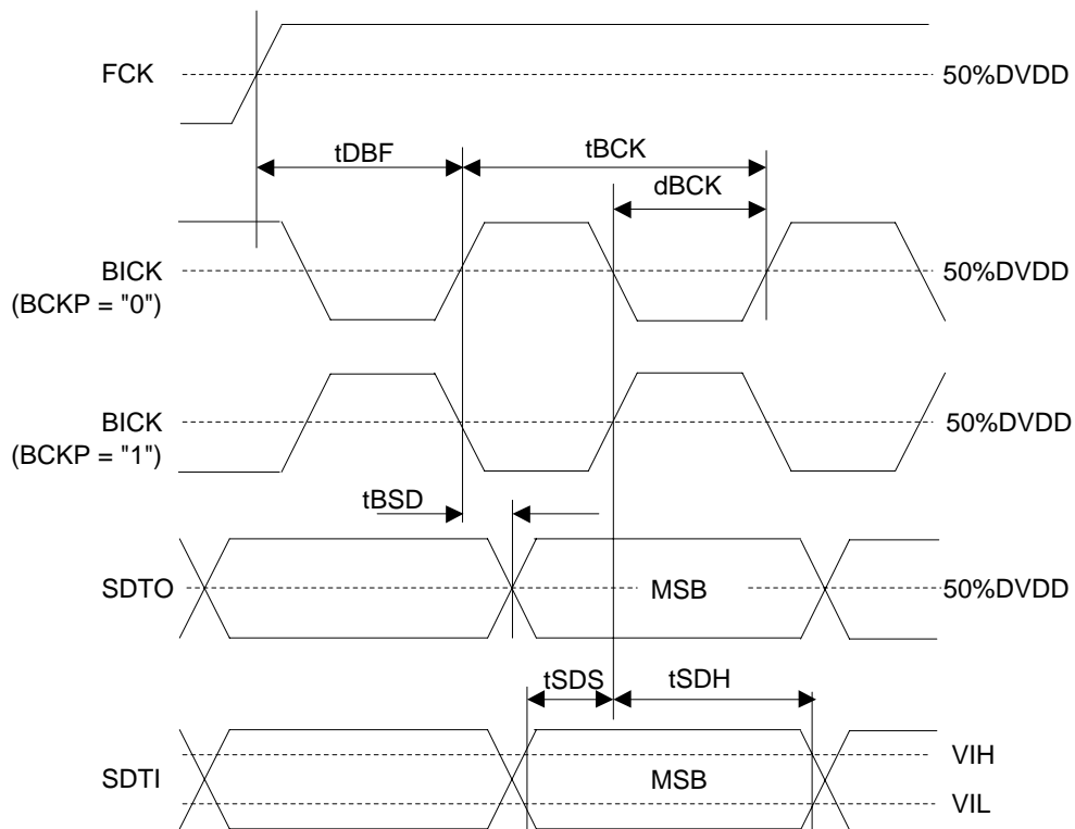
Figure 3. Audio Interface Timing (PLL Master mode & DSP mode: MSBS bit = "0")
