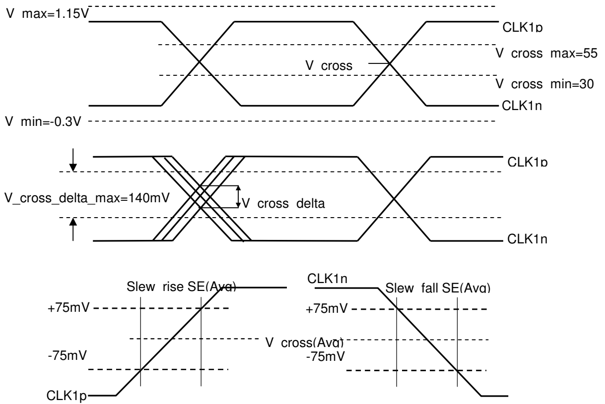
Figure.2 Single ended (SE) measurement waveforms
