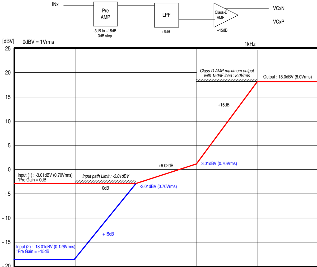
Figure 3. Level Diagram
