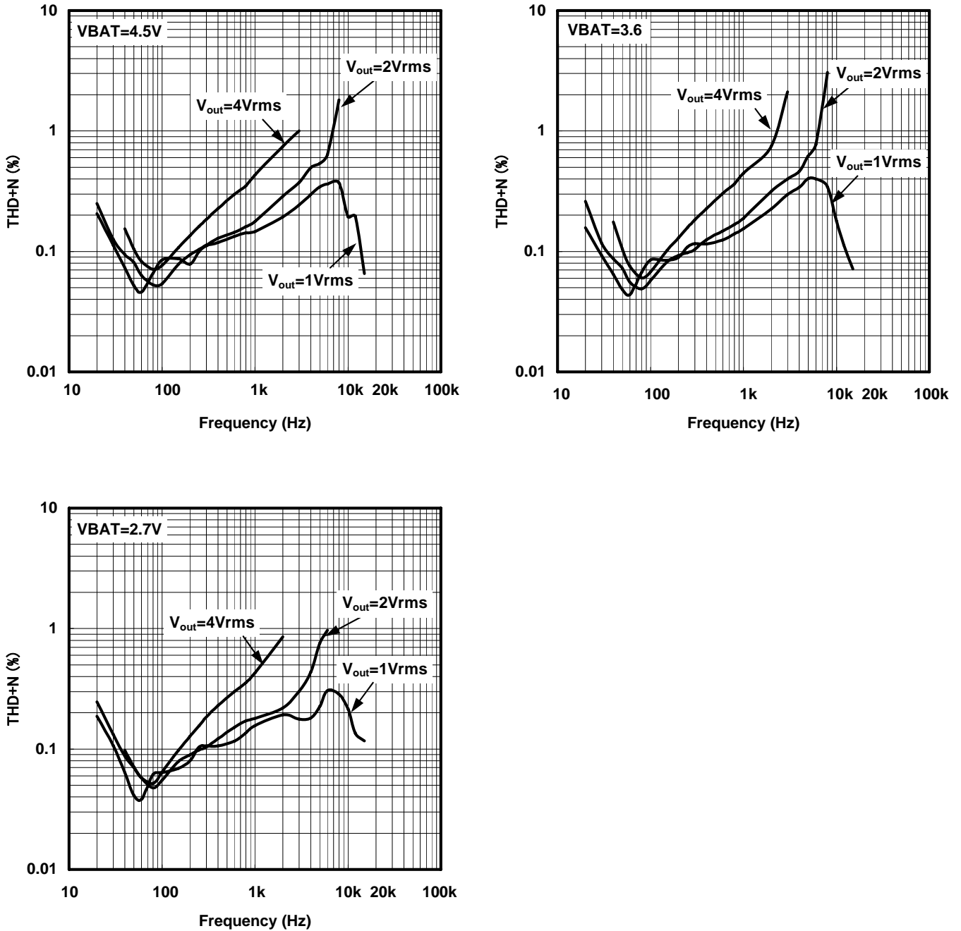
Figure 3. Total Harmonic Distortion Plus Noise vs Frequency
