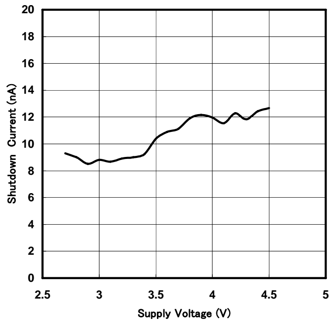
Figure 8. Shutdown Current vs Supply Voltage
