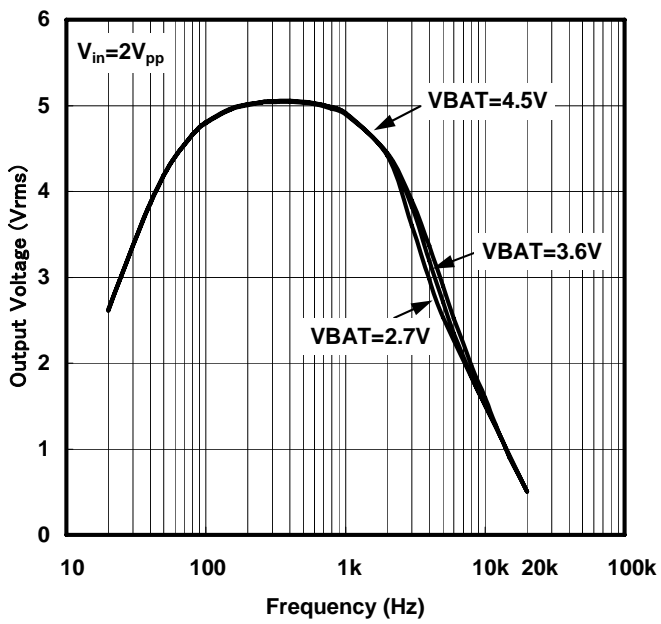
Figure 5. Output Amplitude vs. Frequency
