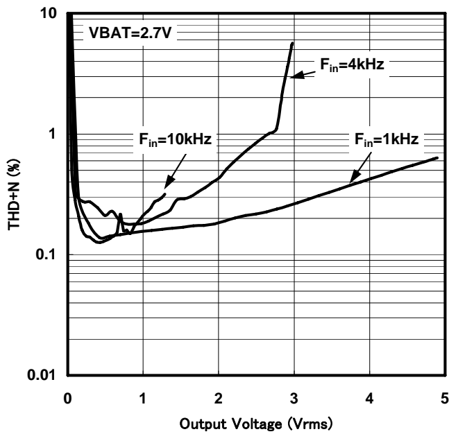
Figure 4. Total Harmonic Distortion Plus Noise vs Output Voltage
