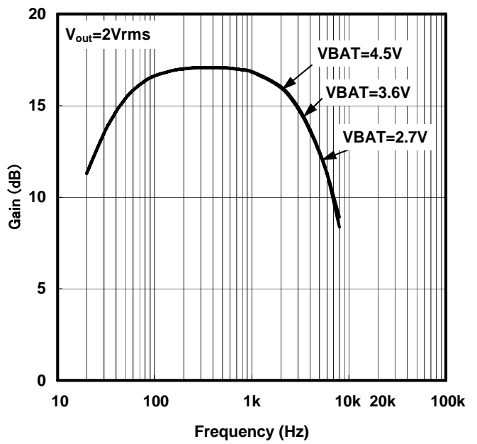
Figure 6. Frequency Response
