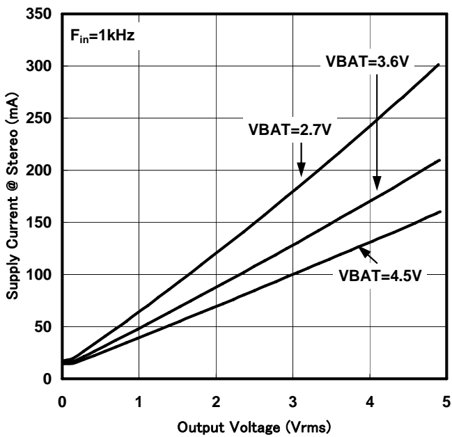
Figure 7. Supply Current vs Output Voltage
