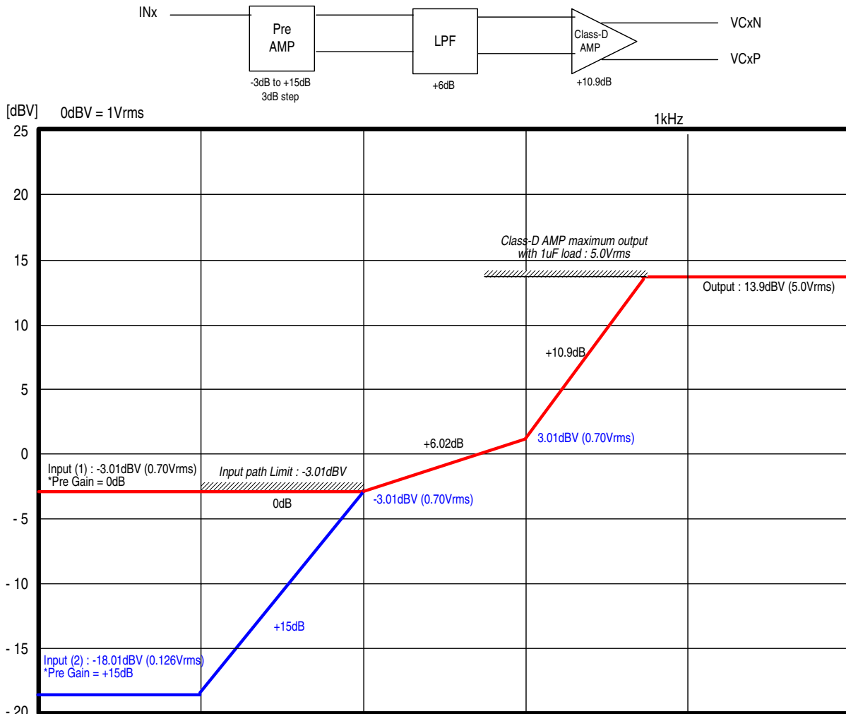
Figure 10. Level Diagram
