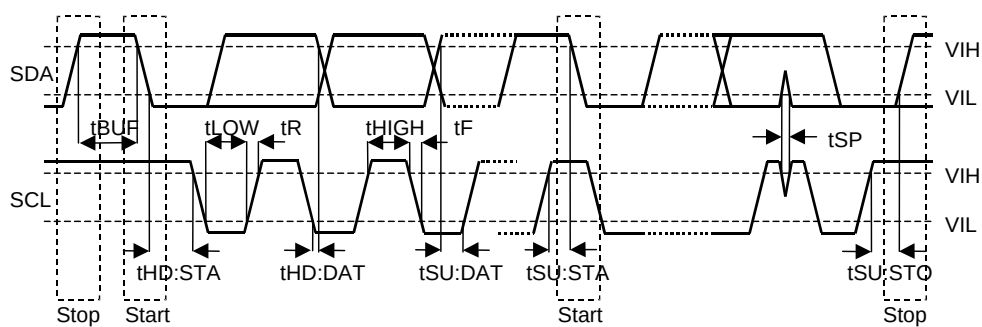
Figure 11. I 2 C-bus Interface
