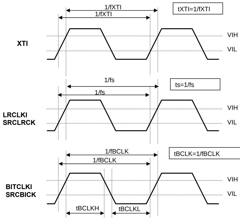
Figure 3. System Clock
