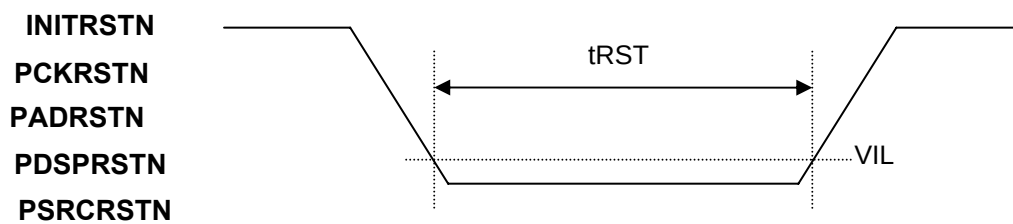
Figure 4. Reset
