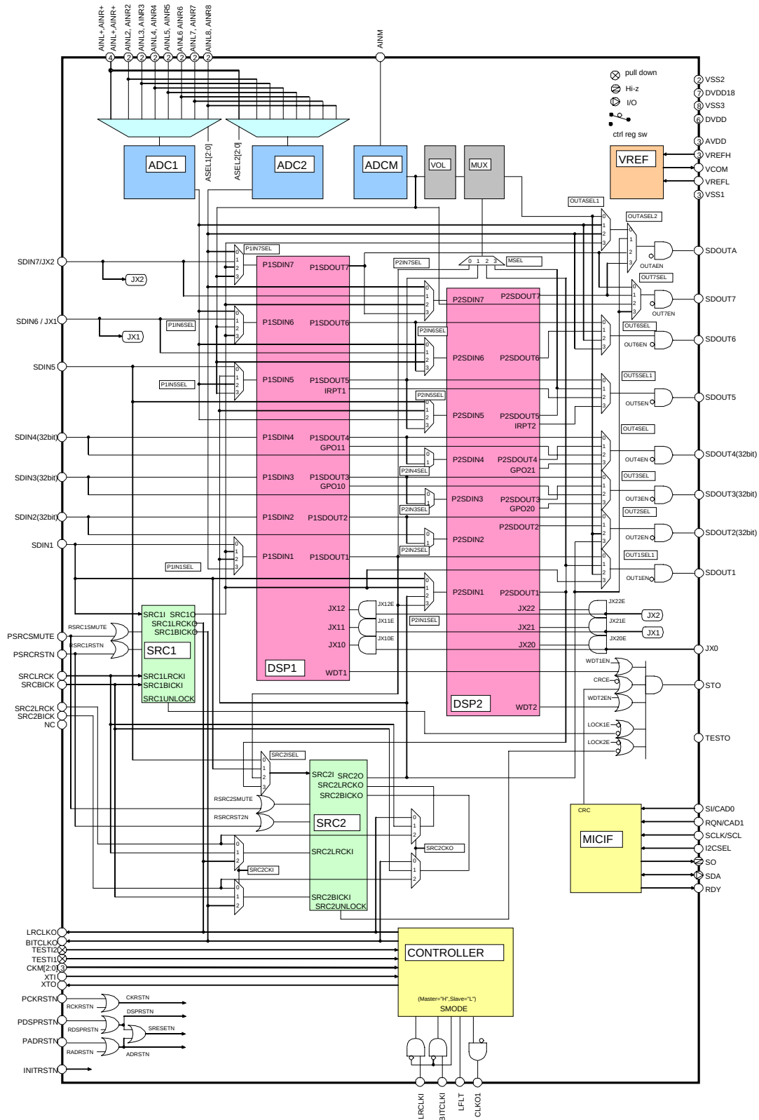
Figure 1. Block Diagram
