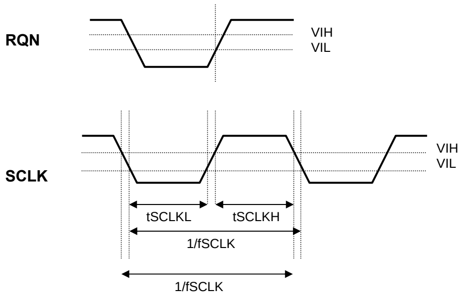
Figure 7. Microprocessor Interface Signal
