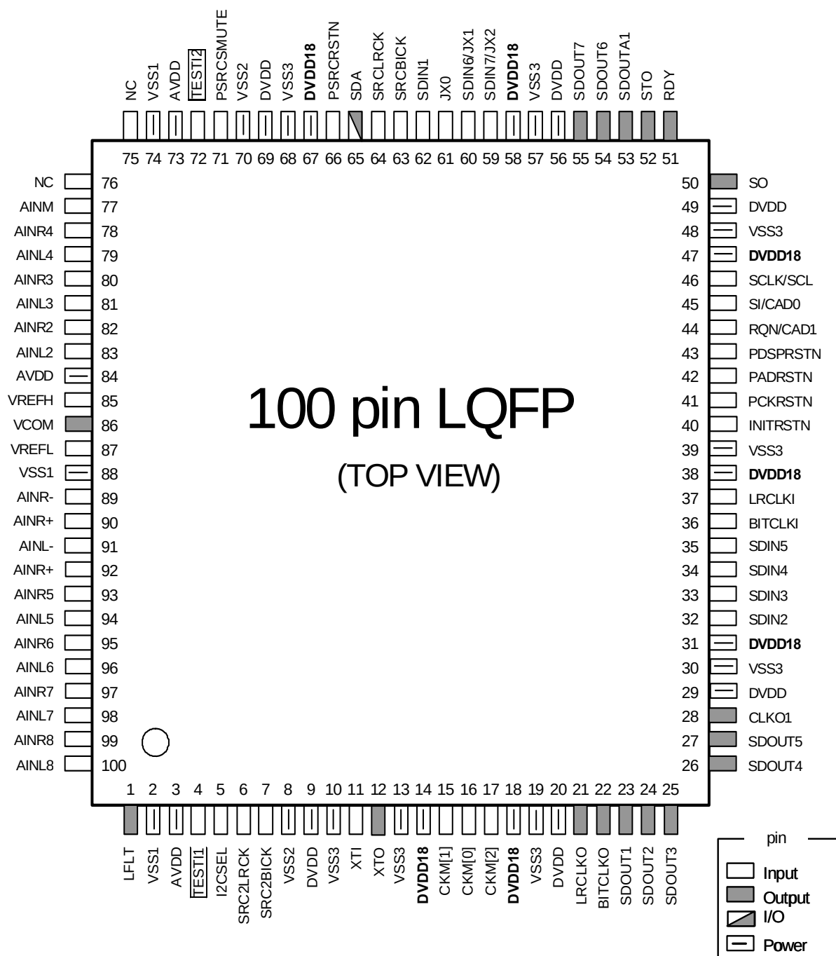
Figure 2. Pin Layout
