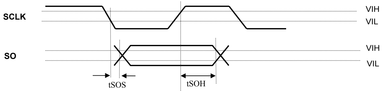
Figure 9. AK7782 → Microprocessor
