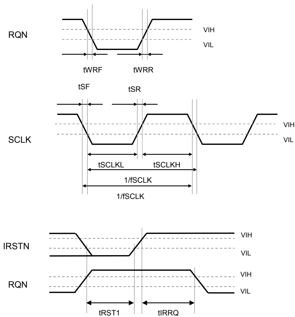
Figure 8. \mu P Interface 1 (SPI)
