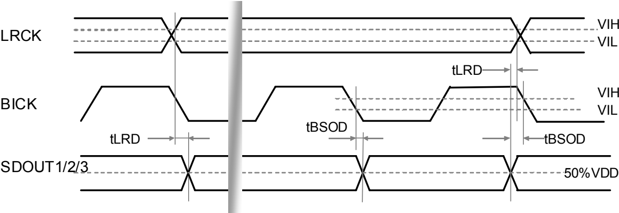
Figure 5. Audio Interface (Slave Mode Output)
