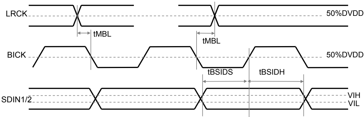
Figure 6. Audio Interface (Master Mode Input)
