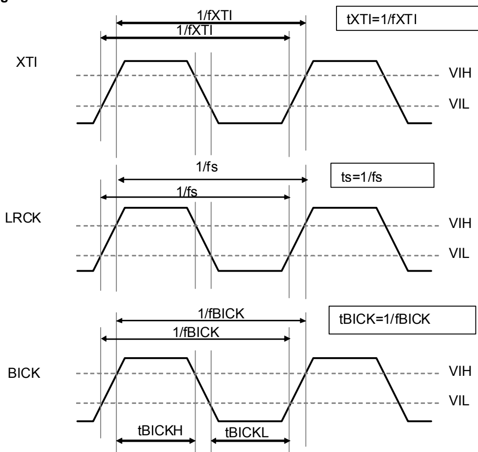
Figure 2. System Clock
