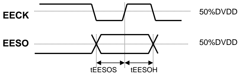
Figure 10. EEPROM Interface 1
