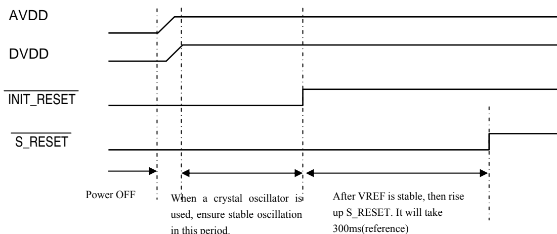
Fig. Power supply startup sequence
