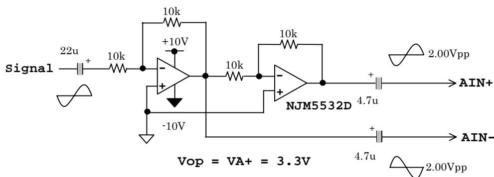
Fig. 1 Example of input buffer circuit (differential input)
