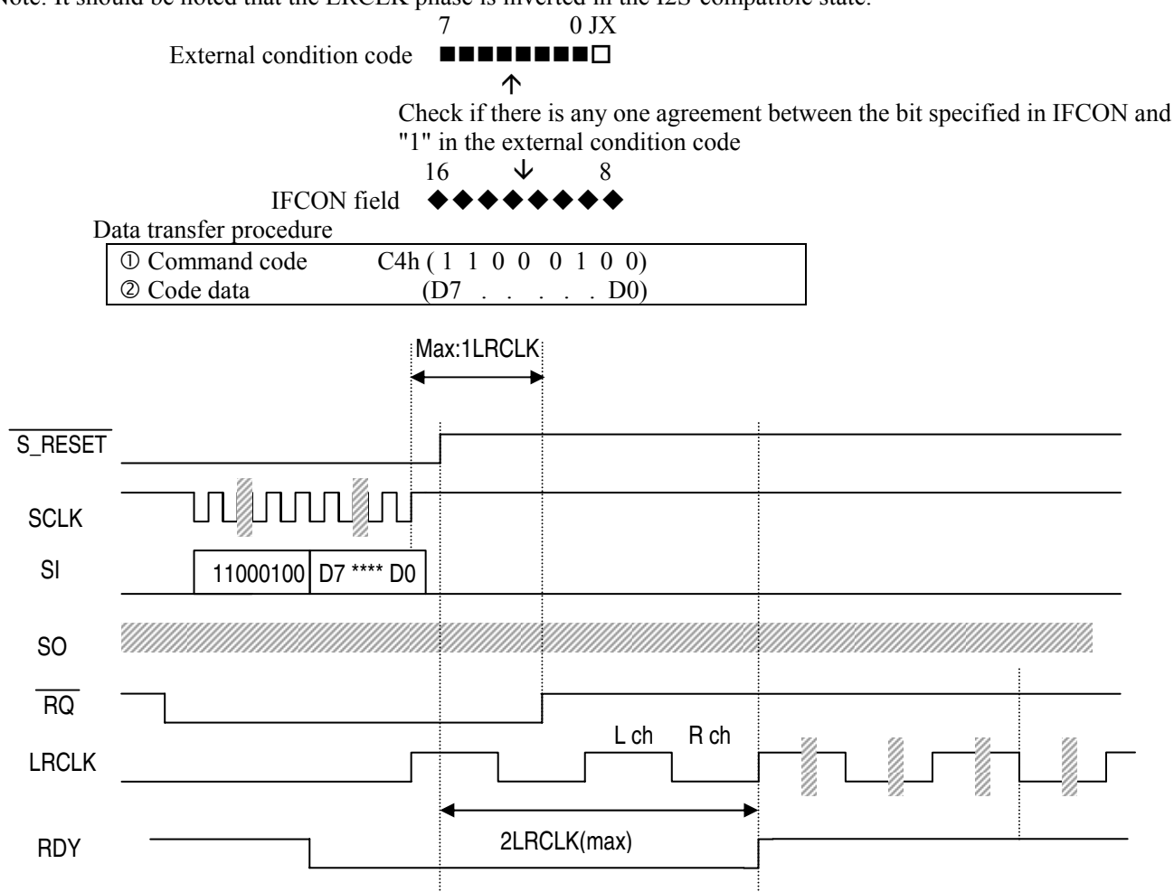
Timing for external conditional jump write operation (during reset phase)
