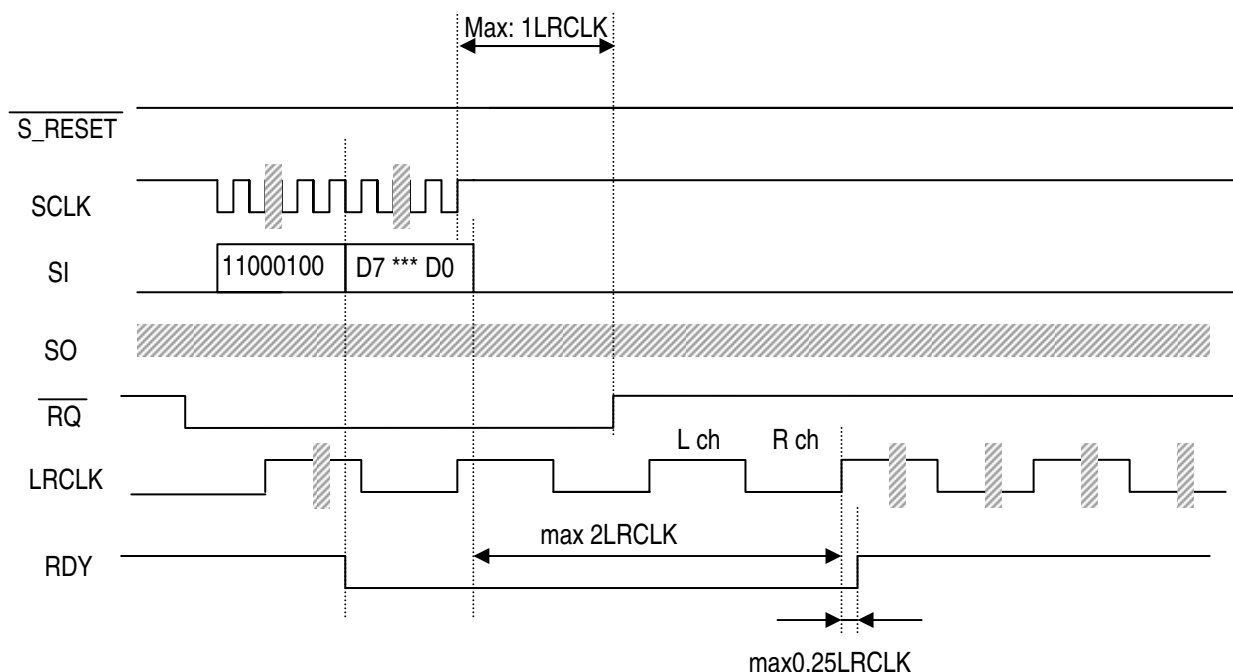
External condition jump write timing (during RUN phase)
