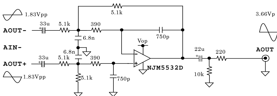
Fig.3 Example of output LPF circuit
