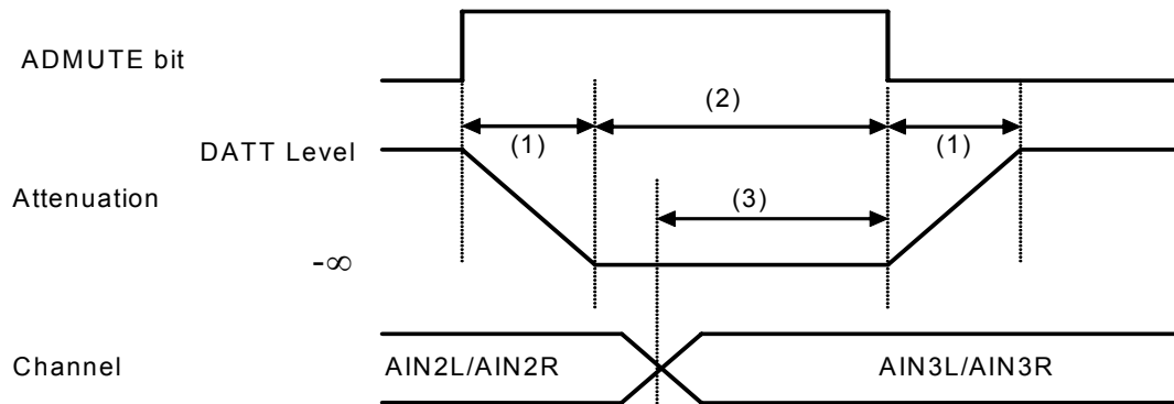
Figure 39. Input Selector Change
