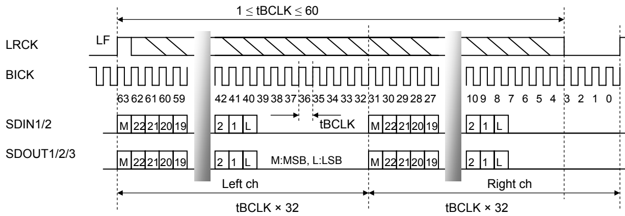
Figure 25. 64fs Long-frame, Rising-edge
