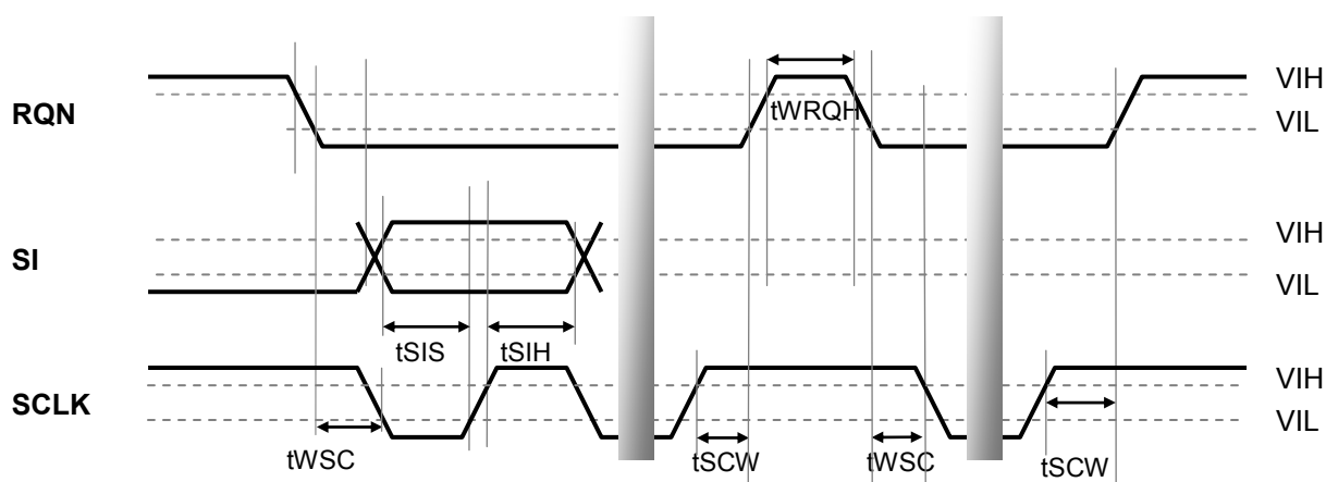
Figure 11. Micro-controller → AK7722
