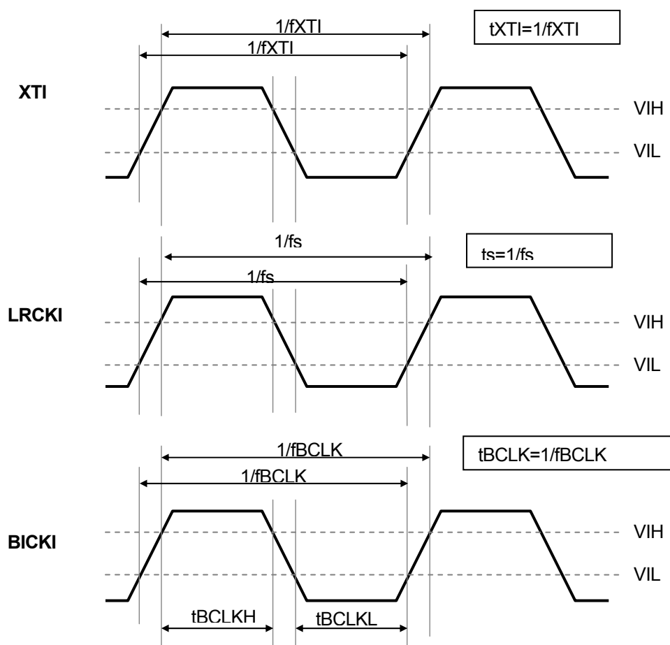
Figure 3. System Clock
