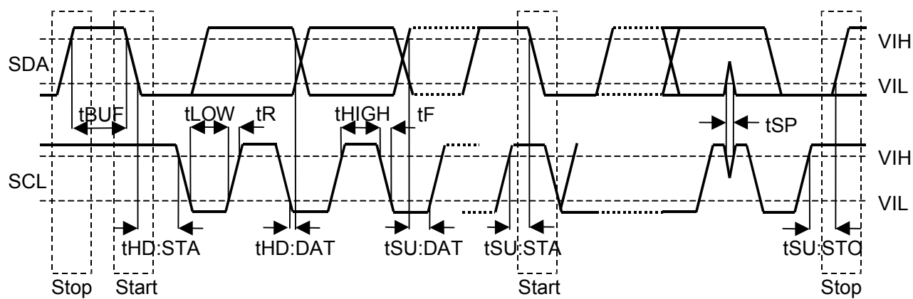
Figure 13. I 2 C-bus Interface
