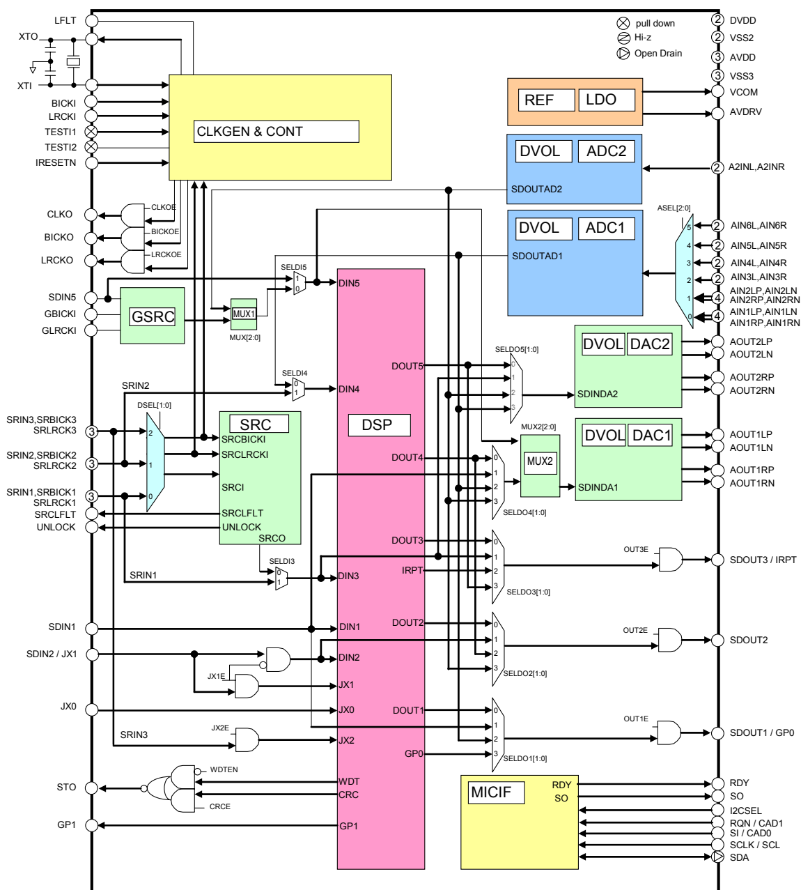
Figure 1. Block Diagram
