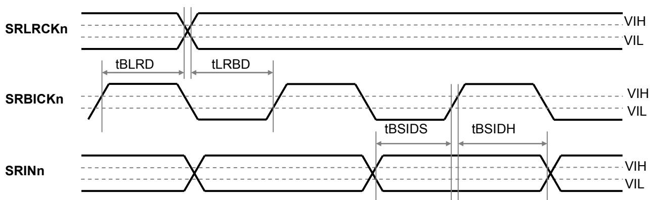
Figure 7. SRC Block Input Interface
