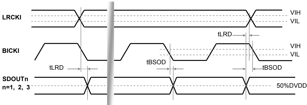
Figure 9. Output Interface in Slave Mode
