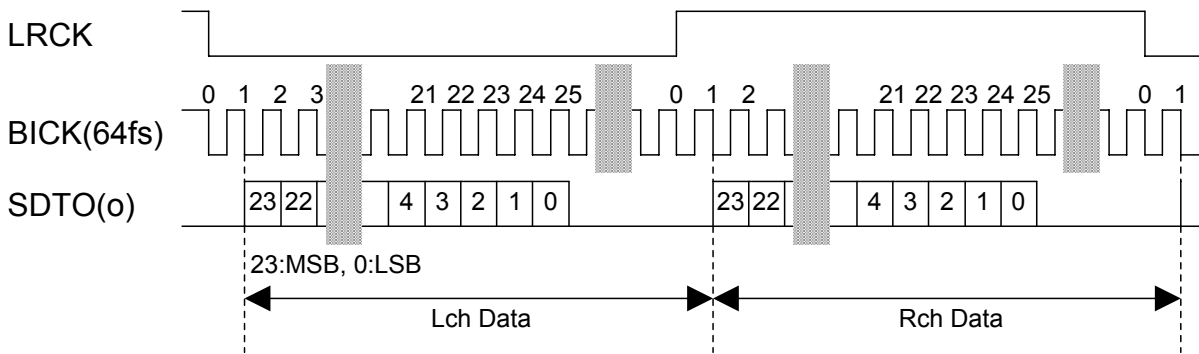
Figure 9. Mode 1 Timing
