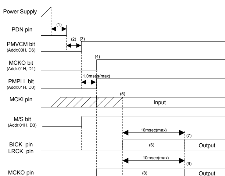
Figure 78. Clock Set Up Sequence (1)
