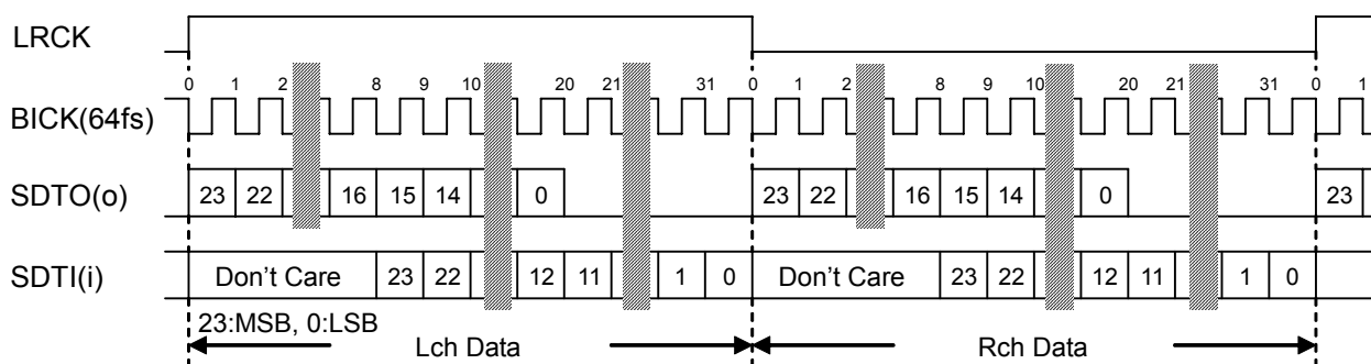
Figure 25. Mode 0 Timing
