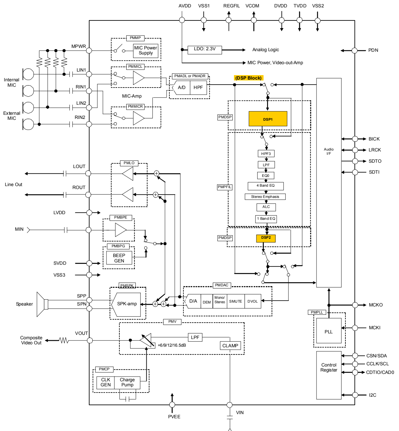
Figure 1. Block Diagram
