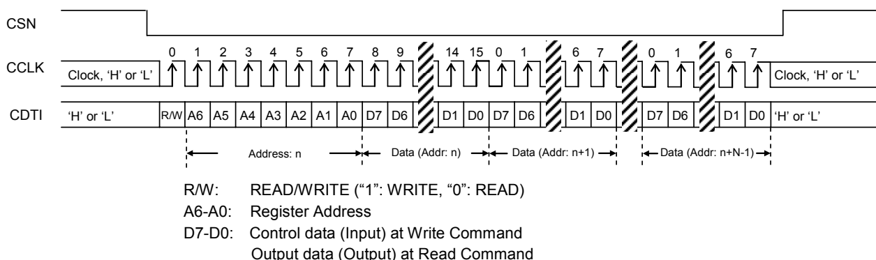
Figure 56. Serial Control Interface Timing 2 (Continuous Writing Mode)
