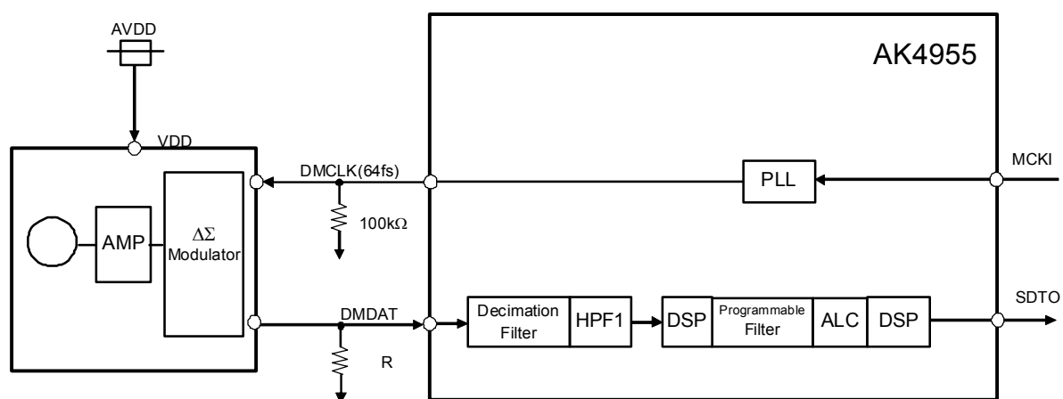
Figure 31. Connection Example of Mono Digital MIC
