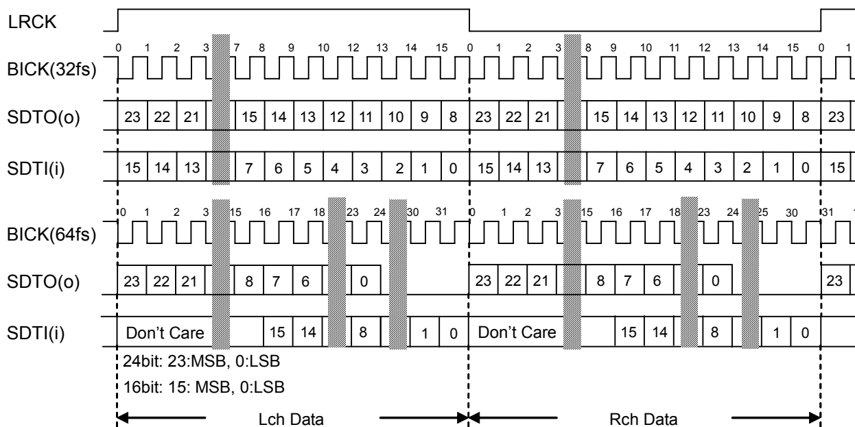
Figure 26. Mode 1 Timing
