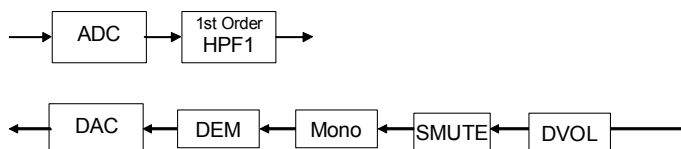
Figure 39. The Path in Recording Mode 3 &amp; Playback Mode 3
