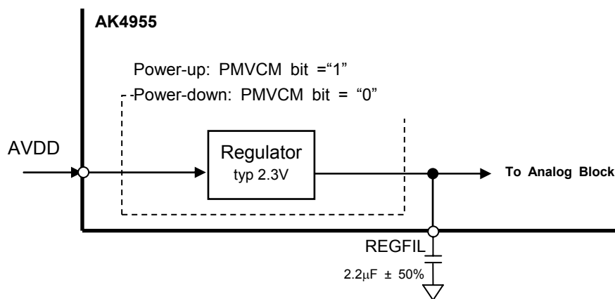
Figure 54 Regulator Block
