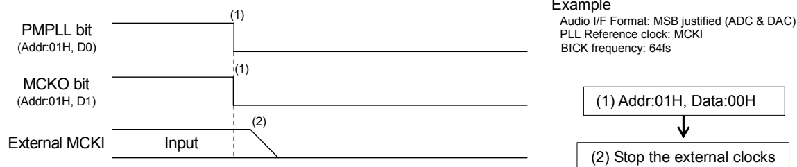
Figure 92. Clock Stopping Sequence (3)
