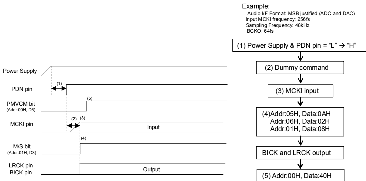
Figure 82. Clock Set Up Sequence (5)
