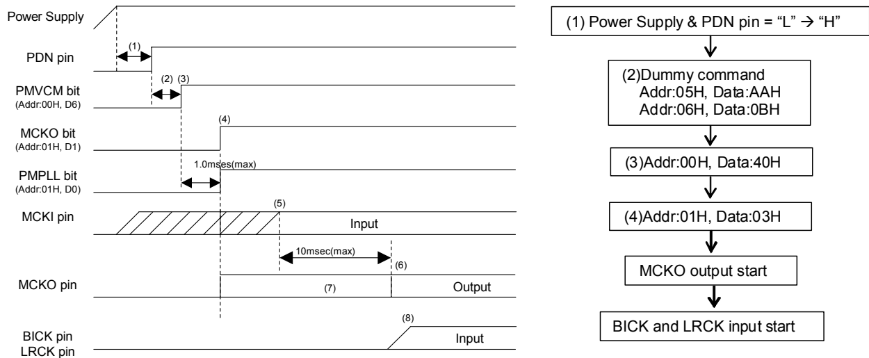
Figure 80. Clock Set Up Sequence (3)
