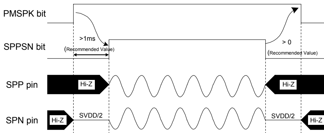
Figure 51. Power-up/Power-down Timing for Speaker-Amp
