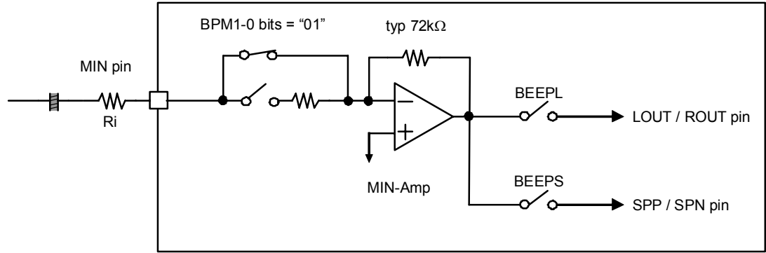
Figure 46. Block Diagram of MIN pin (BPM1-0 bits = “01”)
