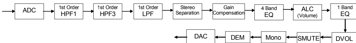
Figure 41. The Path in Loopback Mode 2
