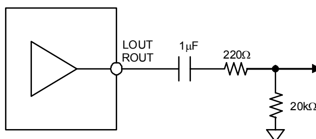
Figure 49. External Circuit for Stereo Line Output (in case of using a Pop Noise Reduction Circuit)
