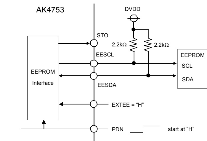
Figure 60. Connection Example of the AK4753 and EEPROM (I 2 C)
