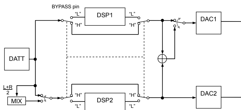
Figure 44. Bypass Mode
