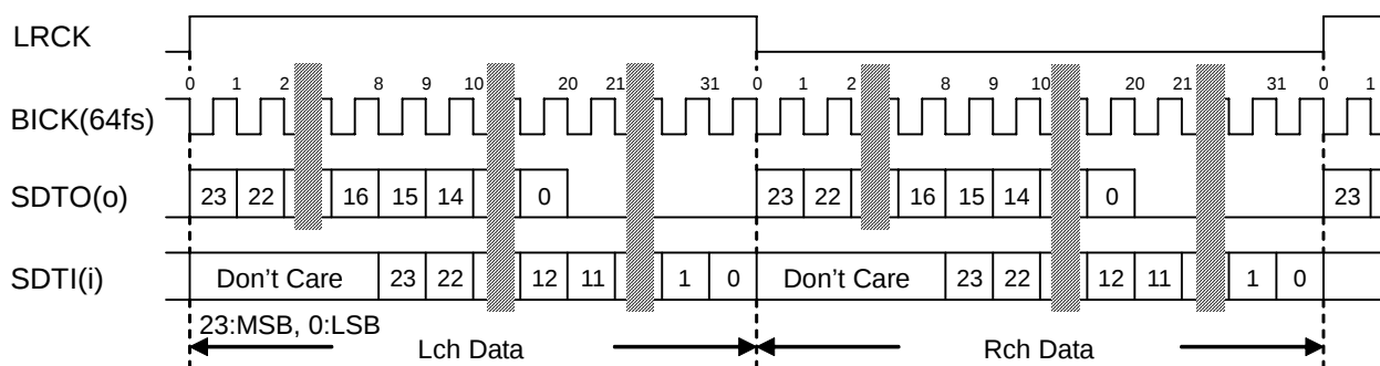
Figure 20. Mode 0 Timing
