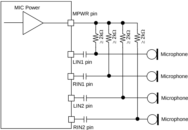
Figure 24. MIC Block Circuit
