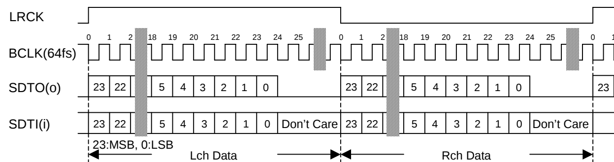
Figure 22. Mode 2 Timing
