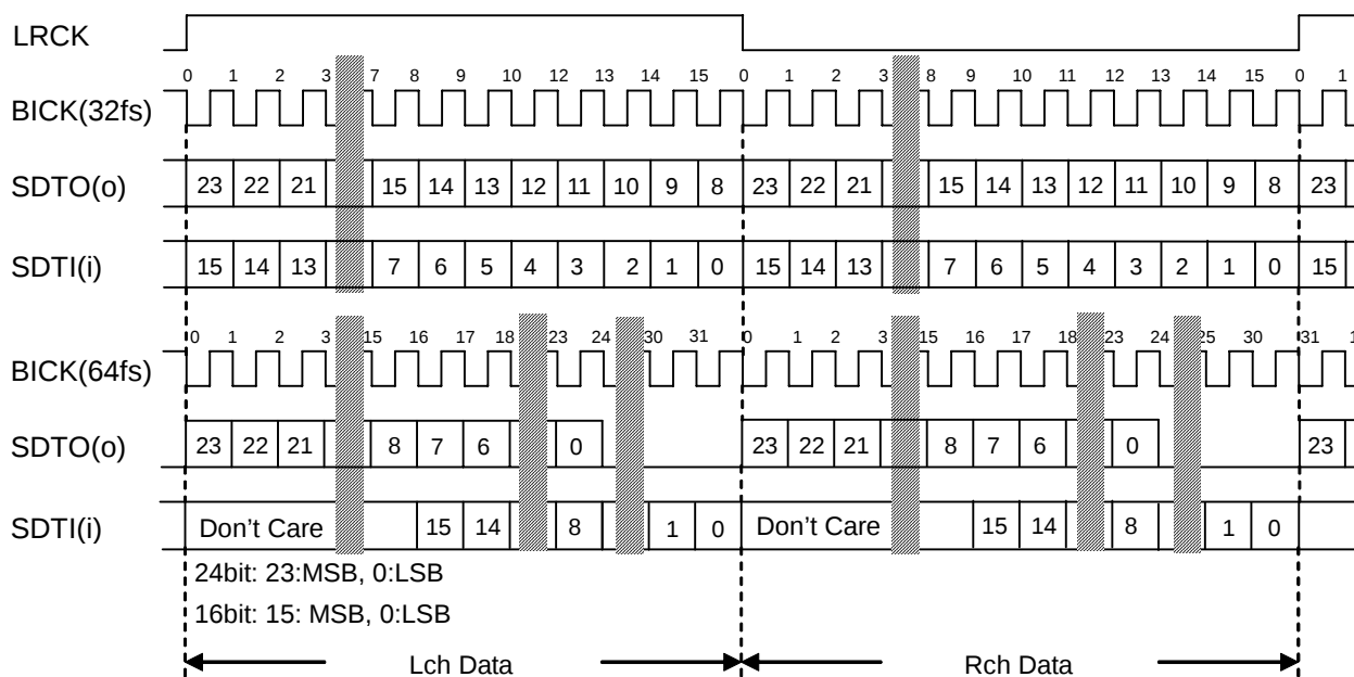
Figure 21. Mode 1 Timing
