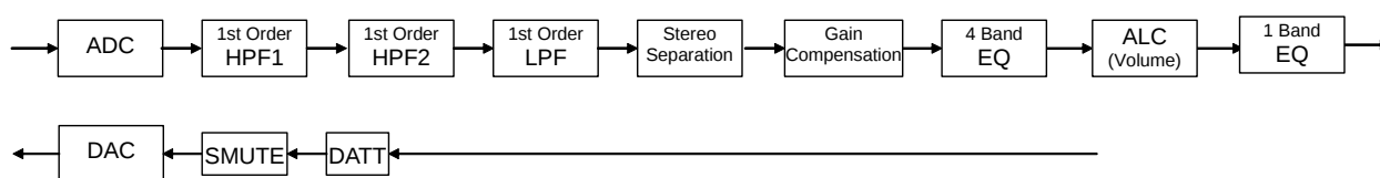
Figure 31. Path at Recording Mode 1 (default)
