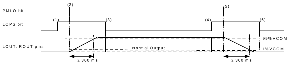
Figure 42. Stereo Line Output Control Sequence (when using Pop Noise Reduction Circuit)
