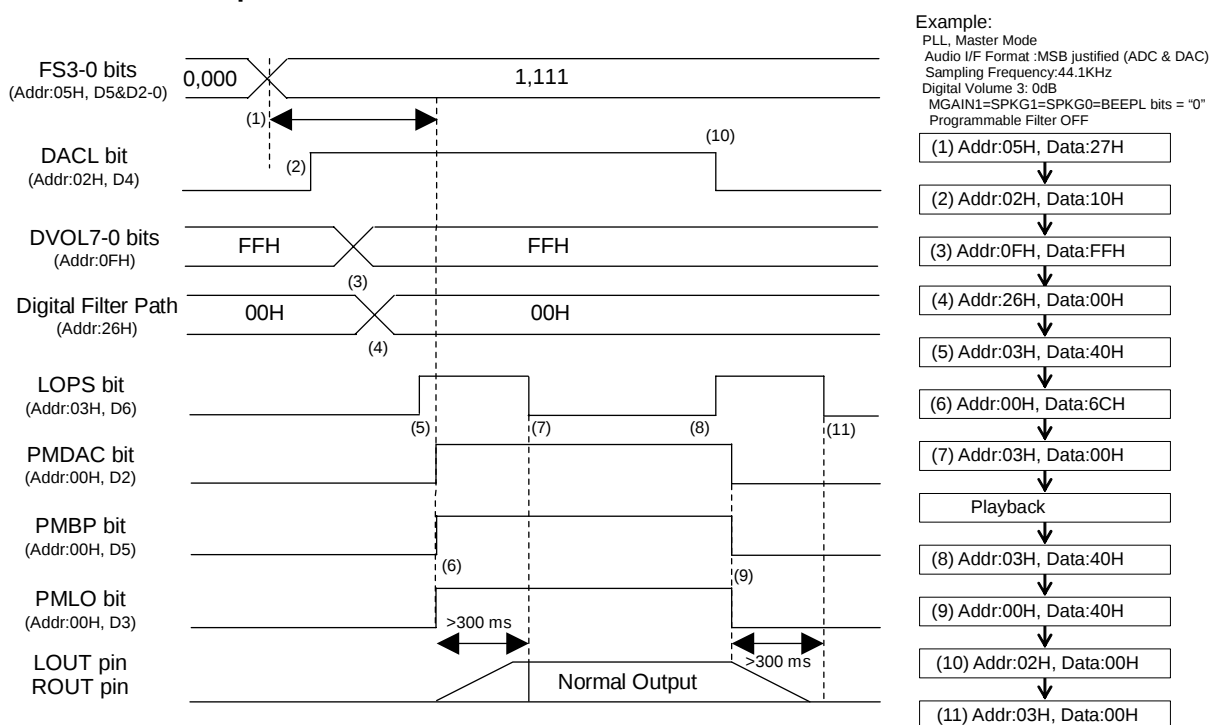
Figure 63. Stereo Lineout Sequence
