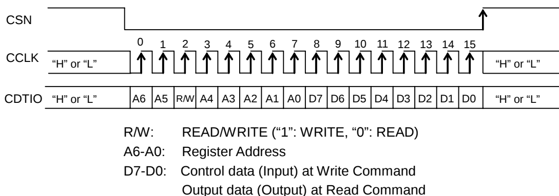
Figure 44. Serial Control I/F Timing
