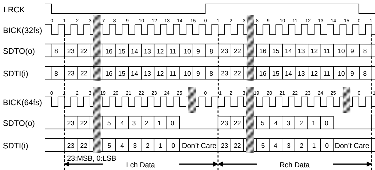
Figure 23. Mode 3 Timing
