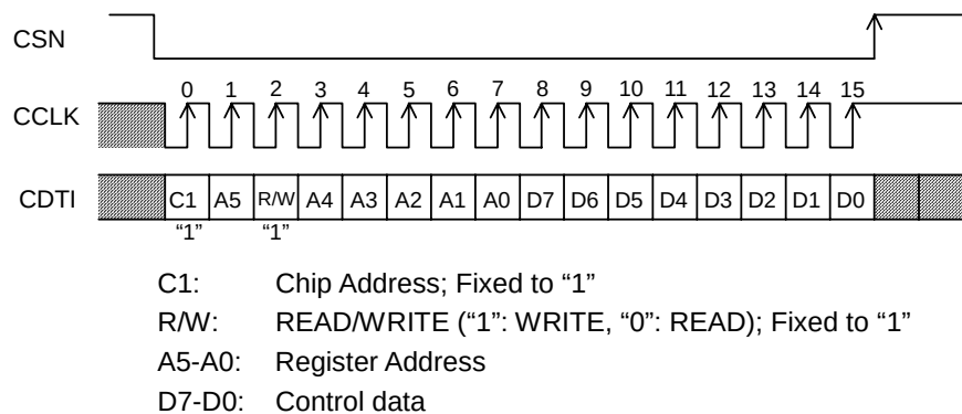
Figure 63. Serial Control I/F Timing
