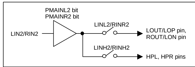
Figure 41. Analog Mixing Circuit (LIN2/RIN2)
