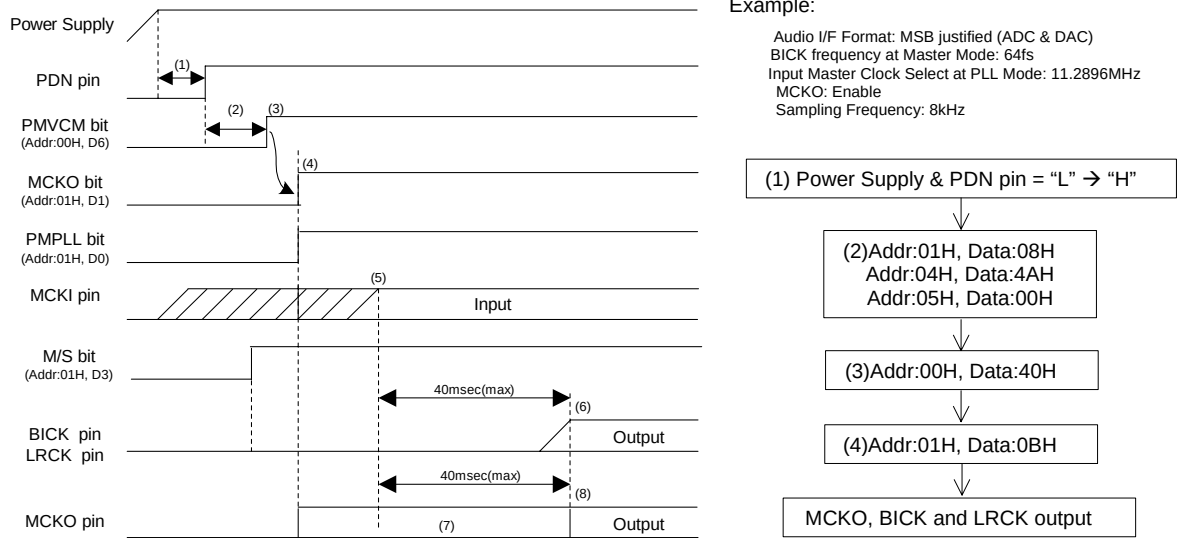
Figure 75. Clock Set Up Sequence (1)
