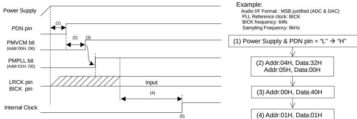
Figure 76. Clock Set Up Sequence (2)
