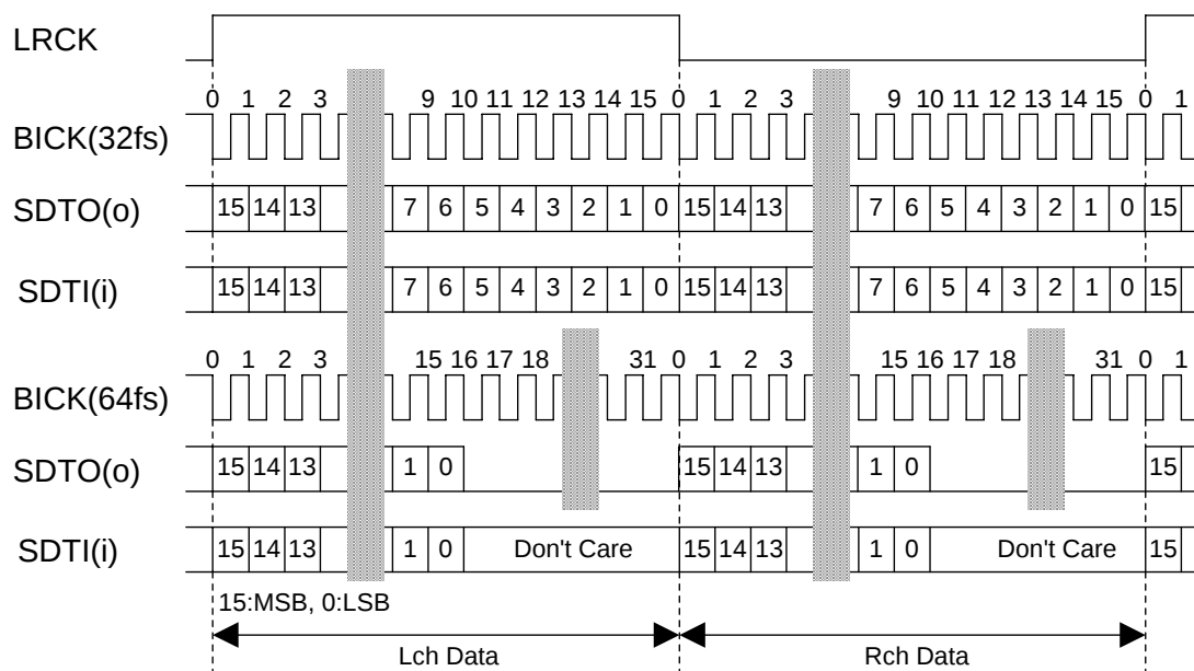
Figure 30. Mode 2 Timing
