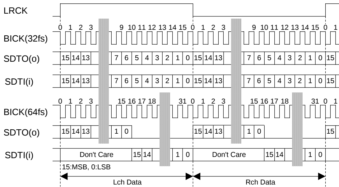
Figure 29. Mode 1 Timing
