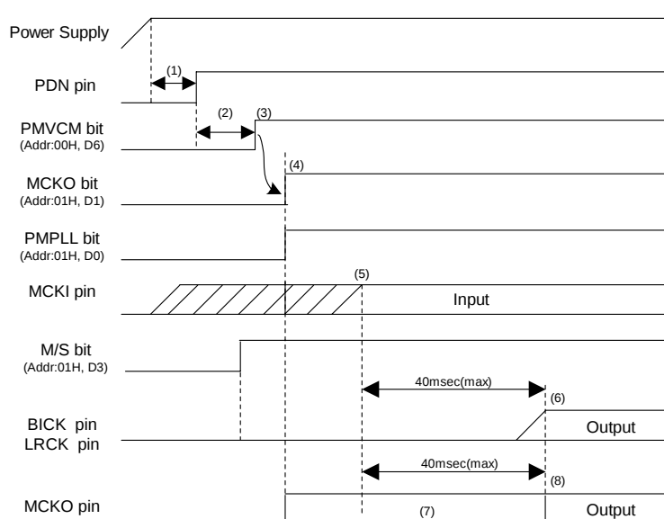
Figure 75. Clock Set Up Sequence (1)
