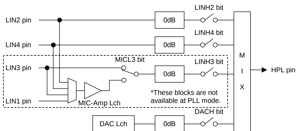
Figure 61. HPL Mixing Circuit (AIN3 bit = "1", HPG bit = "0")
