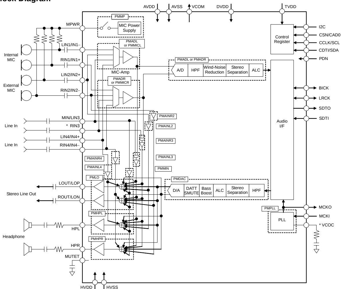
Figure 1. Block Diagram
