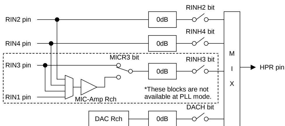
Figure 62. HPR Mixing Circuit (AIN3 bit = "1", HPG bit = "0")
