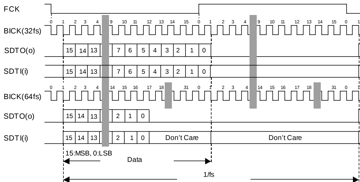
Figure 25. Mode 3 Timing
