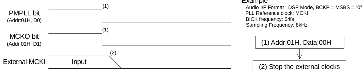
Figure 59. Clock Stopping Sequence (3)
