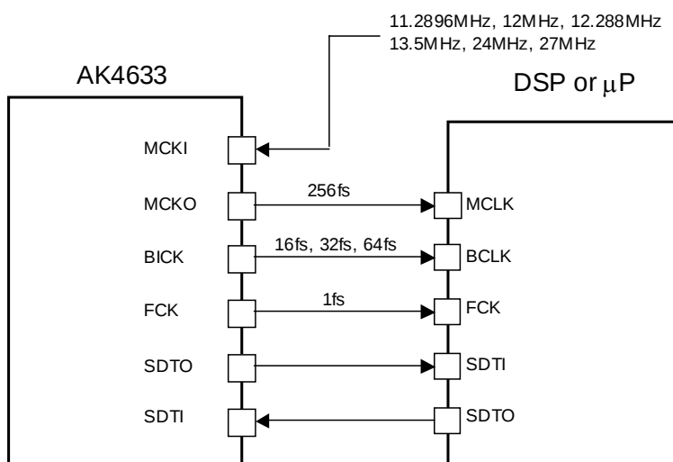
Figure 18. PLL Master Mode
