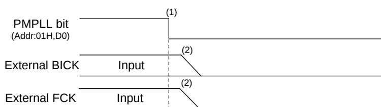
Figure 58. Clock Stopping Sequence (2)
