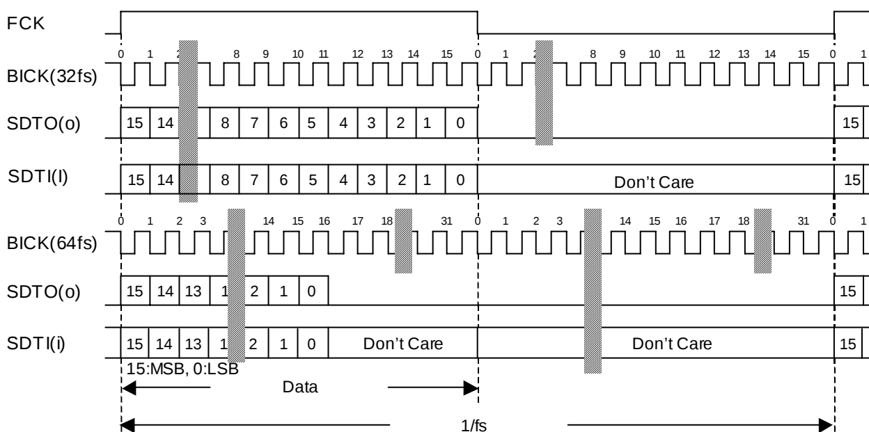
Figure 24. Mode 2 Timing
