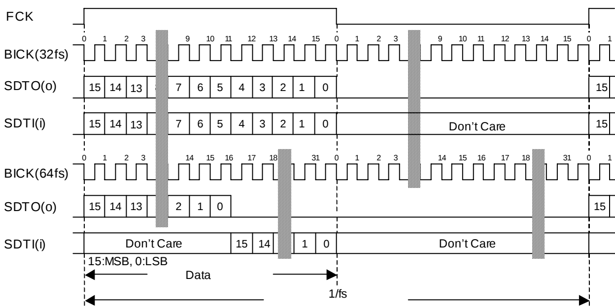
Figure 23. Mode 1 Timing
