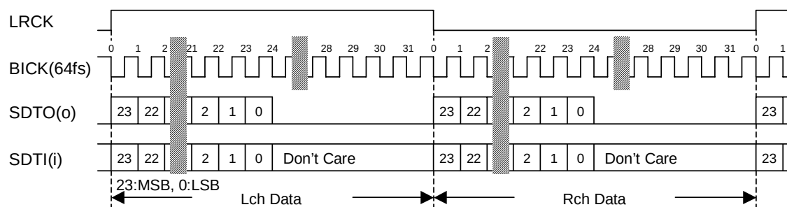
Figure 5. Mode 2 Timing
