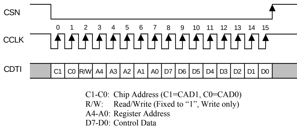
Figure 21. 3-wire Serial Control I/F Timing
