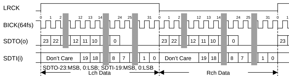
Figure 3. Mode 0 Timing
