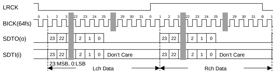
Figure 6. Mode 3 Timing
