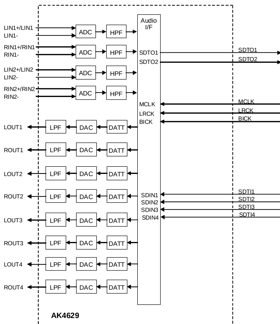
Block Diagram
