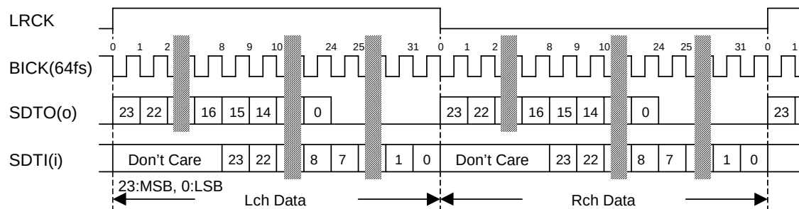
Figure 4. Mode 1 Timing
