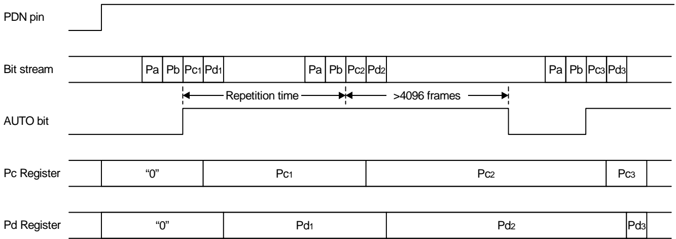
Figure 38. Timing example 1
