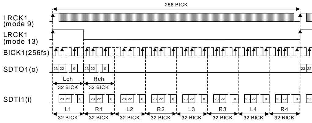
Figure 6. Mode 9/13 Timing
