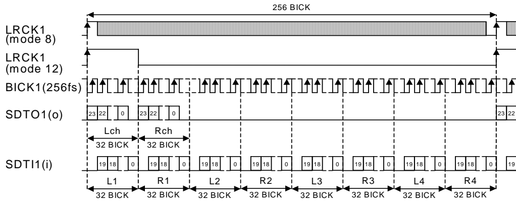
Figure 5. Mode 8/12 Timing
