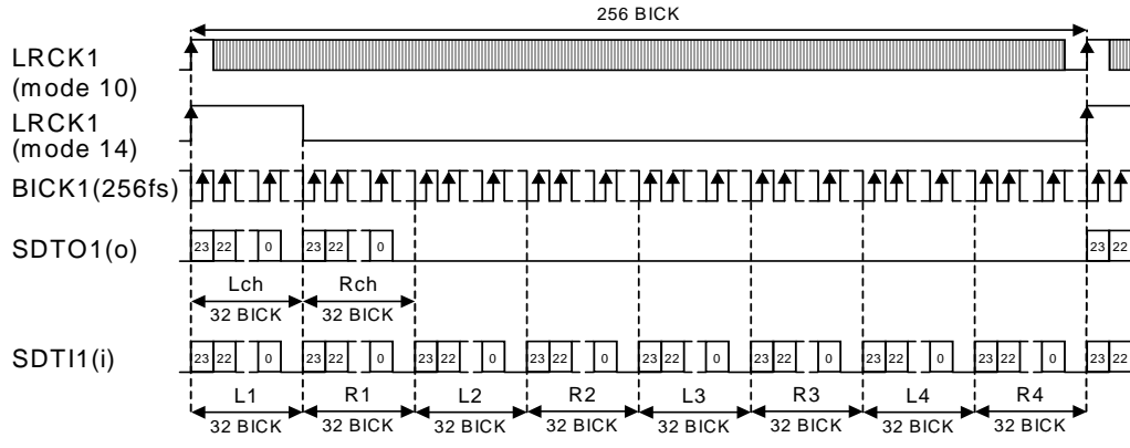
Figure 7. Mode 10/14 Timing
