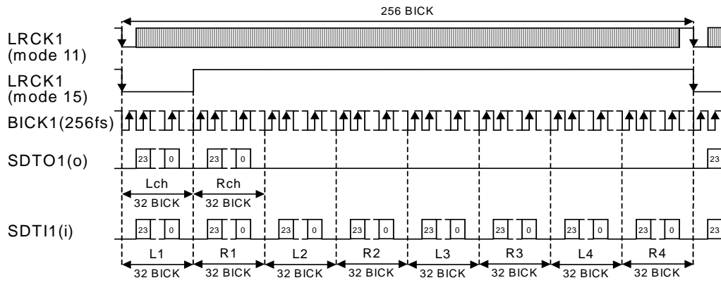
Figure 8. Mode 11/15 Timing
