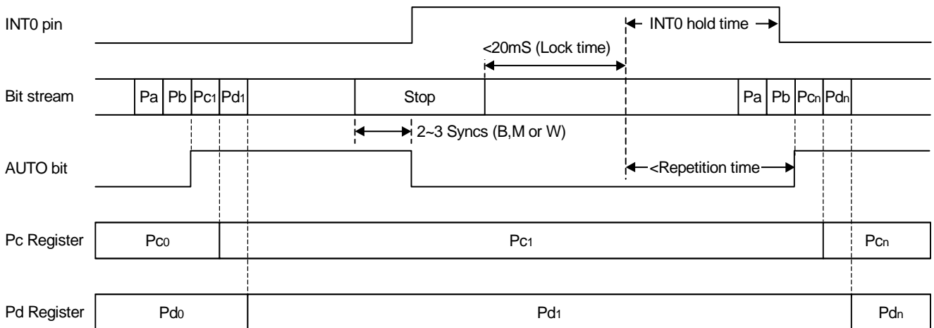
Figure 39. Timing example 2
