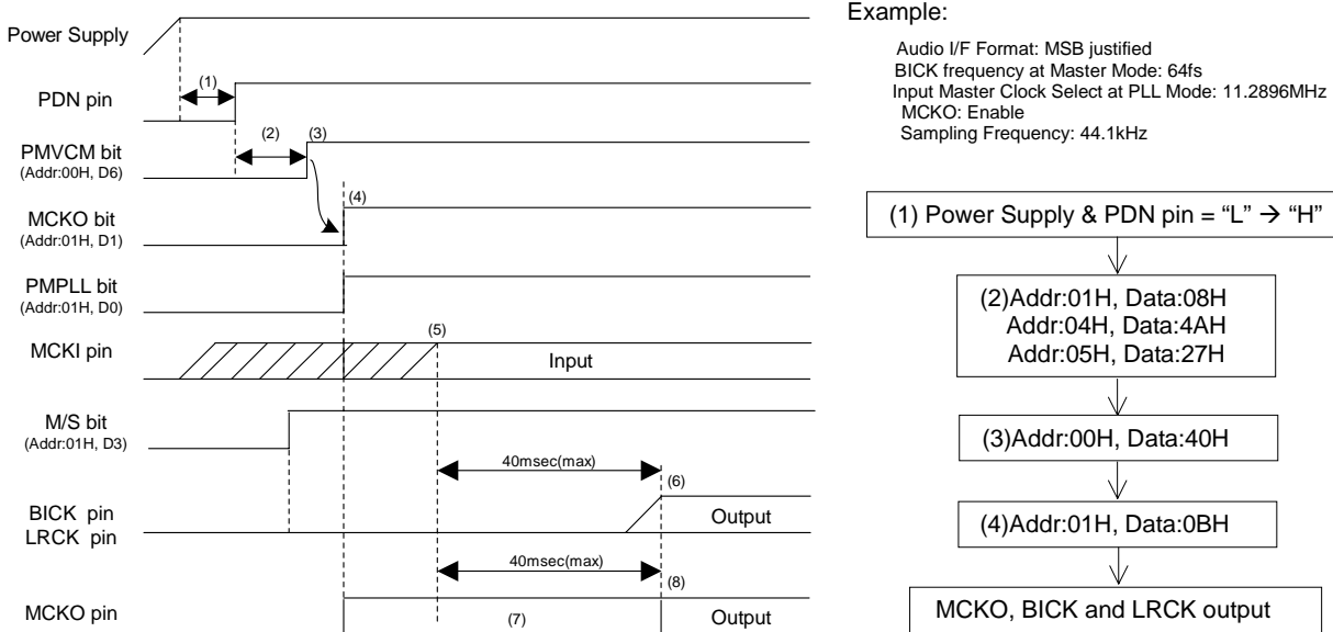
Figure 74. Clock Set Up Sequence (1)
