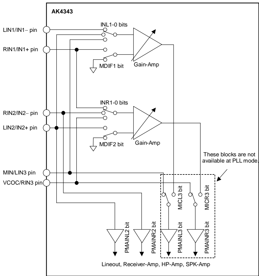
Figure 31. Input Selector
