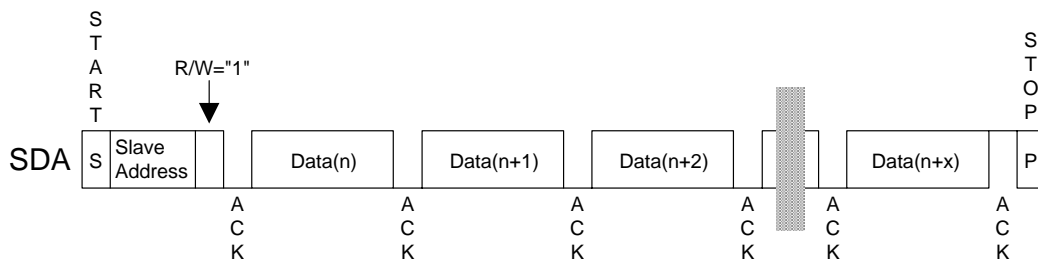
Figure 67. CURRENT ADDRESS READ
