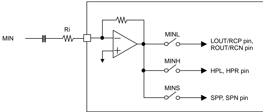
Figure 40. Block Diagram of MIN pin
