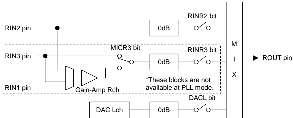
Figure 47. ROUT Mixing Circuit (AIN3 bit = "1", LOVL bit = "0")
