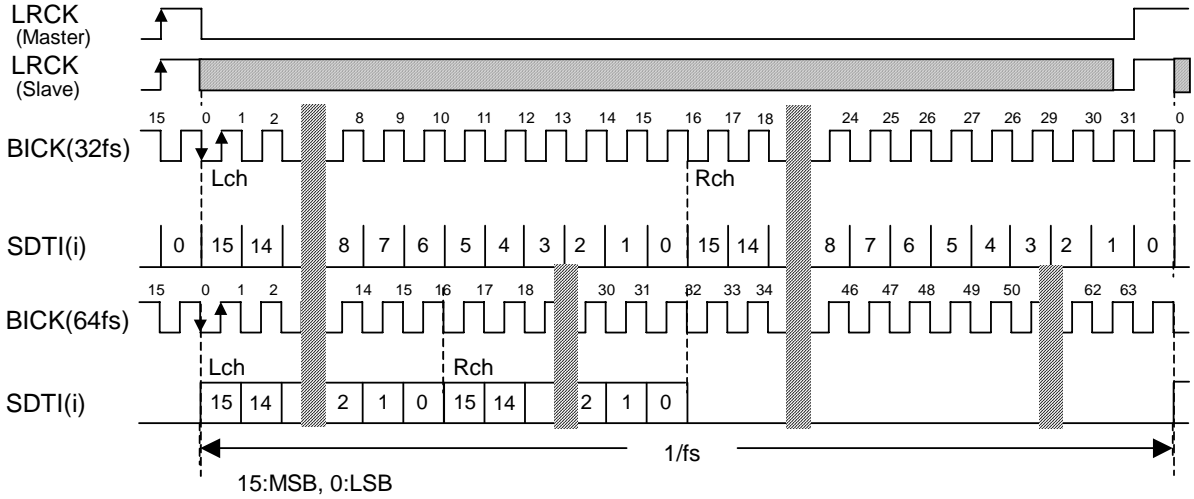
Figure 27. Mode 0 Timing (BCKP = "1", MSBS = "1")
