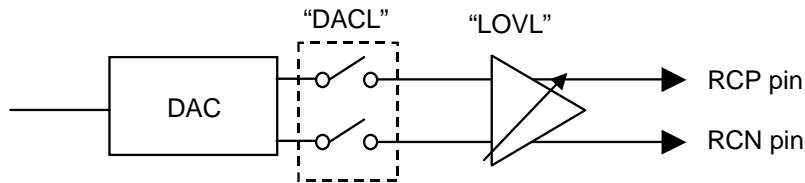
Figure 48. Mono Receiver Output
