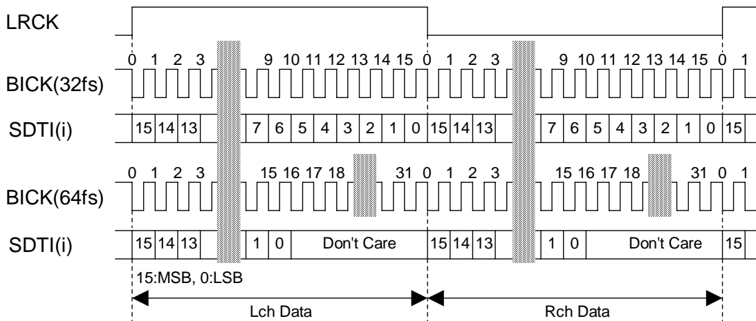
Figure 29. Mode 2 Timing
