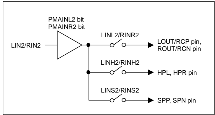
Figure 38. Analog Mixing Circuit (LIN2/RIN2)
