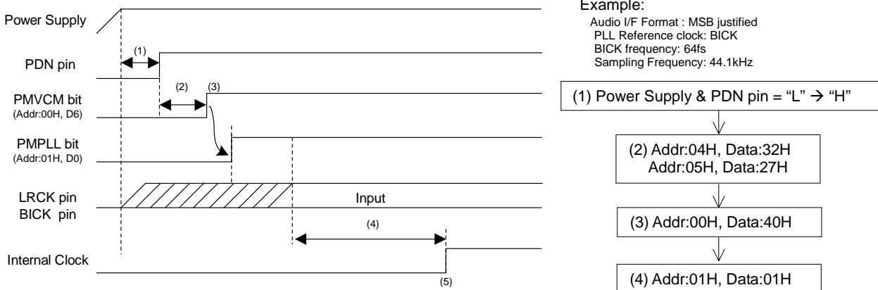
Figure 75. Clock Set Up Sequence (2)
