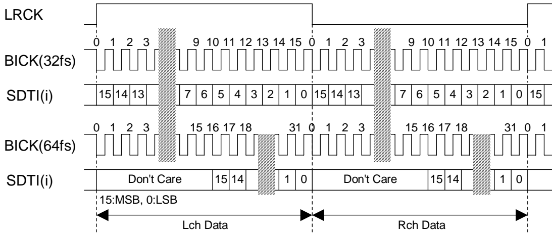
Figure 28. Mode 1 Timing
