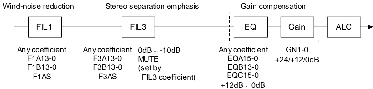
Figure 32. Digital EQ/HPF/LPF
