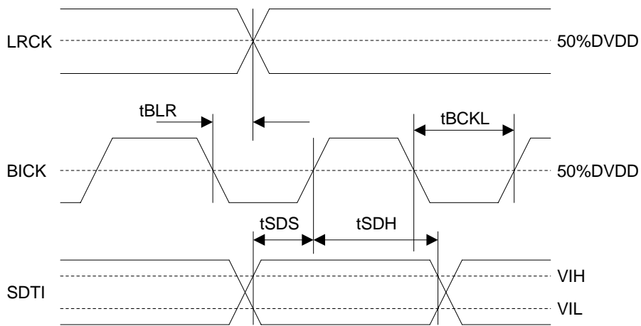
Figure 6. Audio Interface Timing (PLL/EXT Master mode, Except DSP mode)
