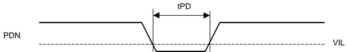
Figure 5. Power-down Timing
