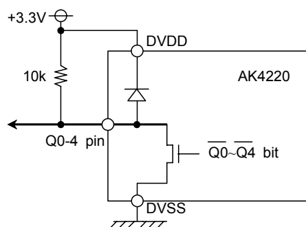
Figure 17. Q0-Q4 Pin Output
