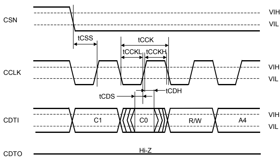
Figure 8. WRITE/READ Command Input Timing (4-wire serial mode)
