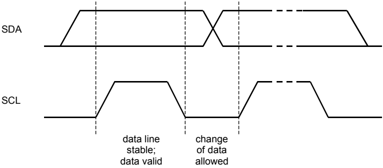
Figure 28. Bit Transfer on the I 2 C-Bus
