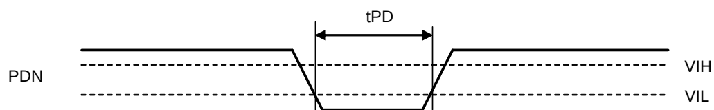
Figure 2. Power-down Timing
