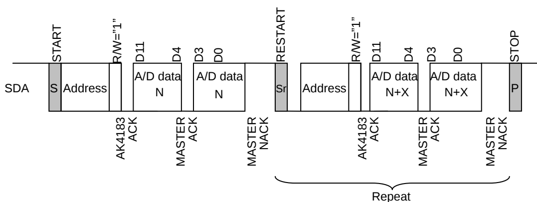
Figure 12 Continuous A/D data Read Sequence
