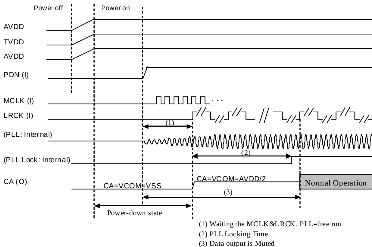
Figure 5. Power-on Sequence
