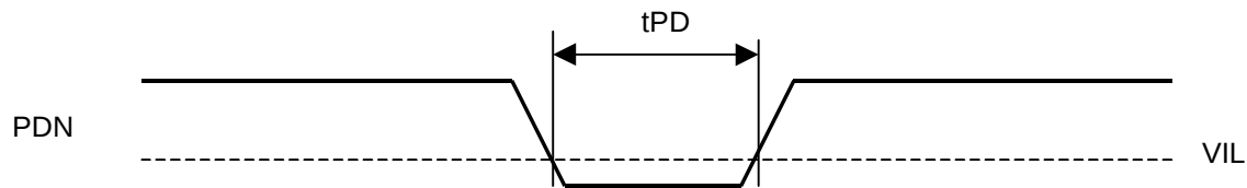
Figure 4. Power-down Timing
