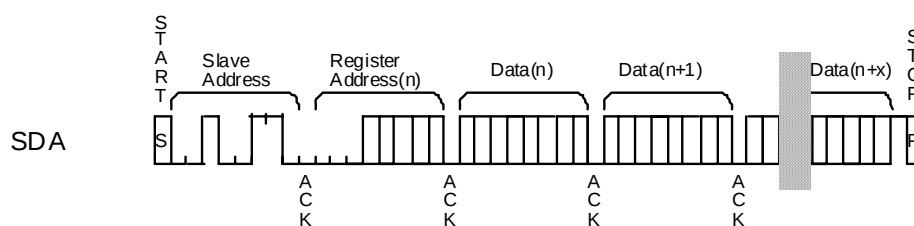
Figure 13. WRITE Operation
