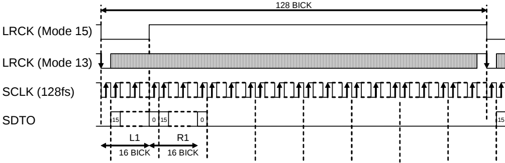
Figure 8. Mode 13, 15 Timing (TDM128B mode, I²S Compatible)
