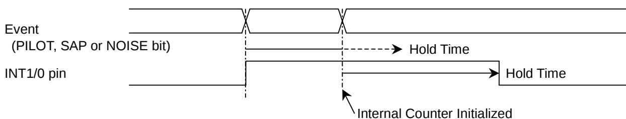
Figure 14. INT pin Timing
