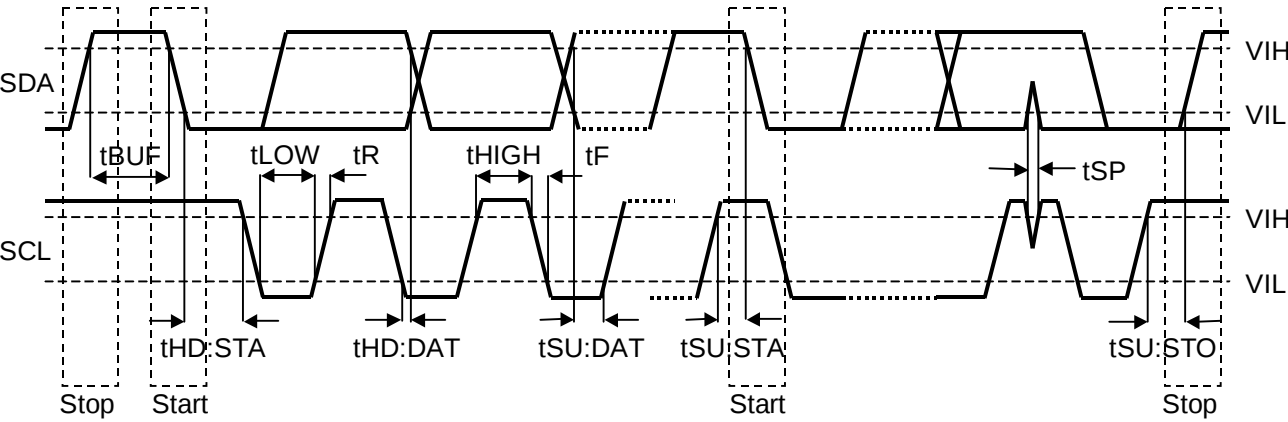
I²C Bus mode Timing
