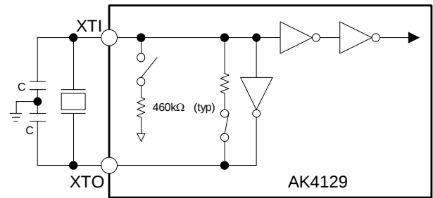
Figure 21. X'tal Mode
