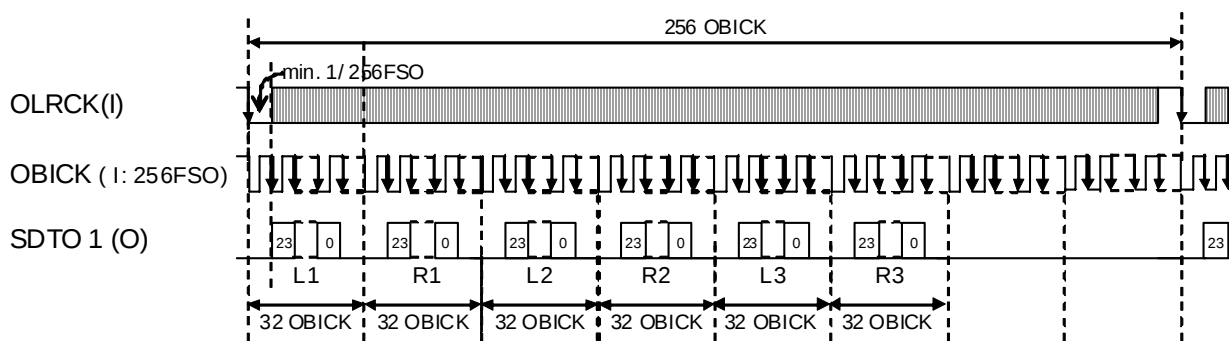
Figure 31. TDM 256 mode 24bit I²S Compatible Timing at Slave Mode (SDTO2-3: “L” outputs)
