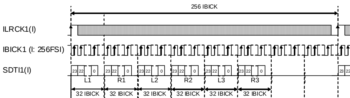
Figure 19. Mode 5 Timing (TDM, 24bit, MSB justified, SDTI2-3: Don't care)
