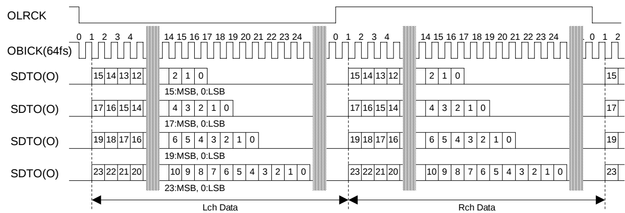
Figure 27. Stereo Mode I²S Compatible Timing
