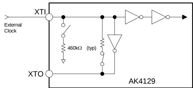
Figure 22. External Clock (OMCLK) mode
