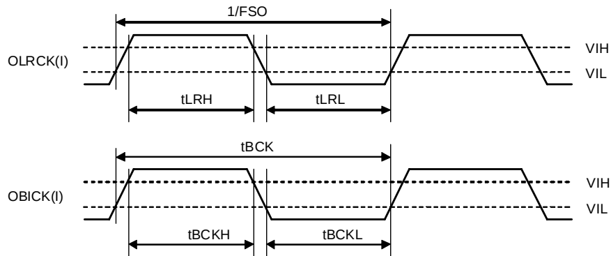
Figure 7. OLRCK, OBICK, Clock Timing (Slave Mode)
