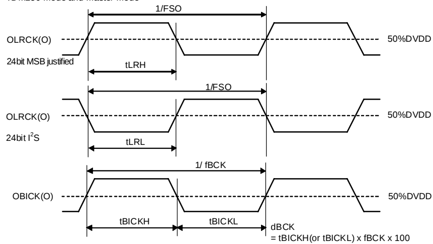
Figure 8. OLRCK, OBICK, Clock Timing (Master Mode)
