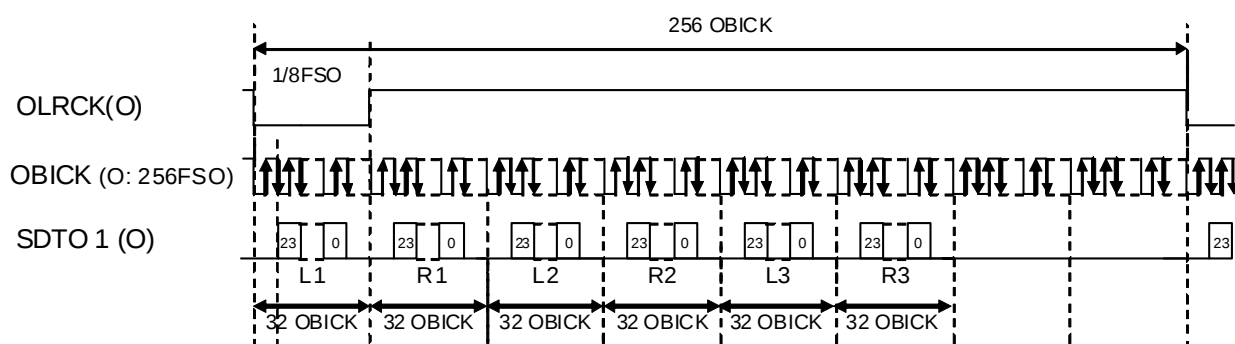
Figure 30. TDM 256 mode 24bit I²S Compatible Timing at Master Mode (SDTO2-3: “L” outputs)
