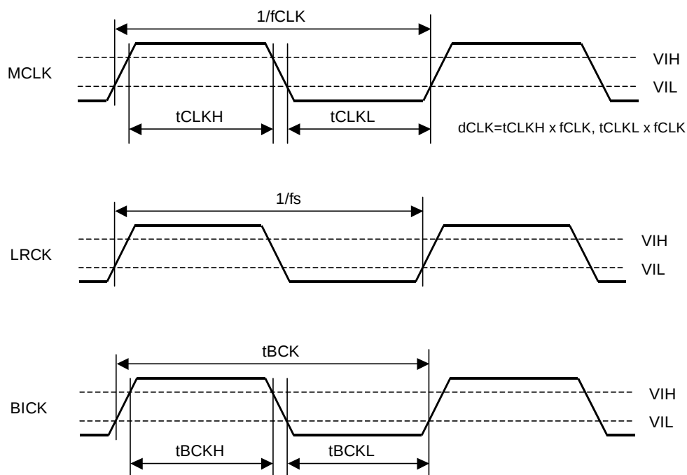
Figure 1. Clock Timing
