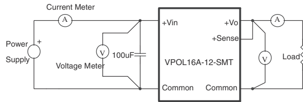
Figure 11. VPOL16A-12-SMT Series Test Setup
