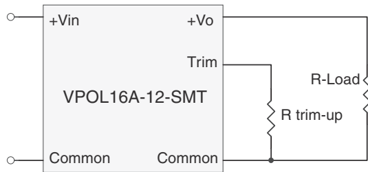
Figure 13. Trim-up Voltage Setup The value of Rtrim-up defined as:
