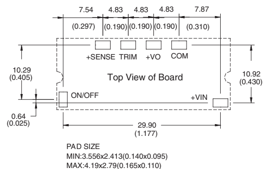
Figure 5. Recommended VPOL16A-12-SMT Footprint
