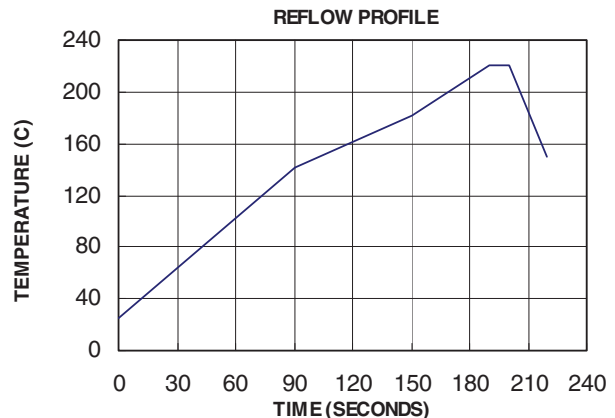
Figure 15 VPOL16A-12-SMT Reflow Profile
