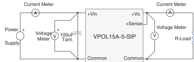
Figure 12. VPOL15A-5-SIP Series Test Setup
