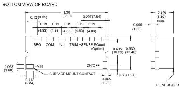
Figure 18 VPOL10A-12W-SMT Mechanical Outline Diagram
