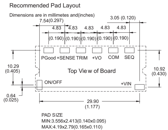
Figure 8. Recommended VPOL10A-12W-SMT Footprint
