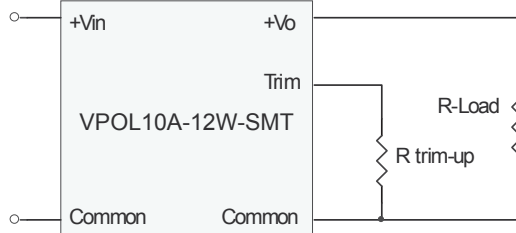
Figure 15. Trim-up Voltage Setup
