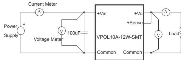
Figure 13. VPOL10A-12W-SMT Series Test Setup
