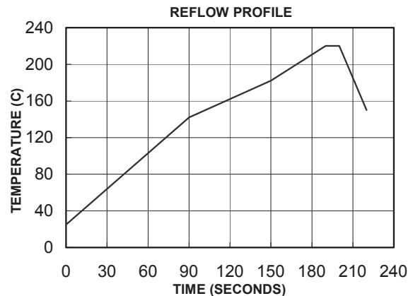
Figure 17 VPOL10A-12W-SMT Reflow Profile
