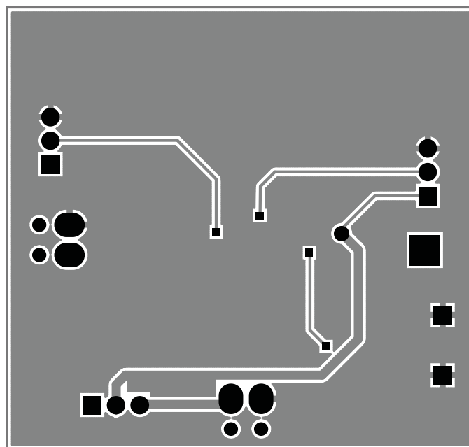
Figure 4: AAT2557 Evaluation Board Bottom Side Layout.
