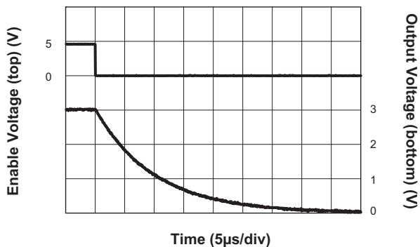
LDO Turn-Off Response Time (I OUT = 100mA)
