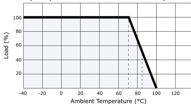
output power vs. ambient temperaure
